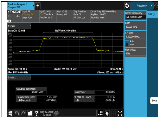
Band5-5MHz-QPSK-20625-25RB#0
