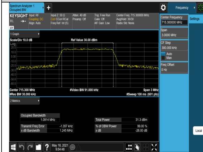
Band12-1.4MHz-16QAM-23095-6RB#0
