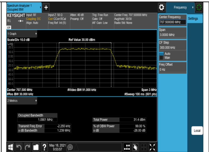
Band12-1.4MHz-16QAM-23017-6RB#0
