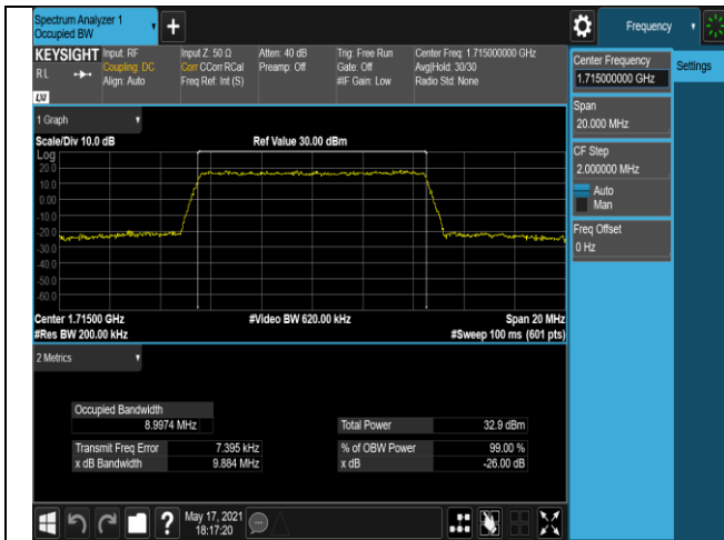
Band4-10MHz-QPSK-20350-50RB#0
