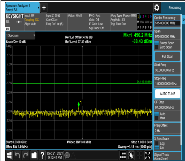
Band2-20MHz-16QAM-18700-1RB#0-Range1:30~1000MHz
