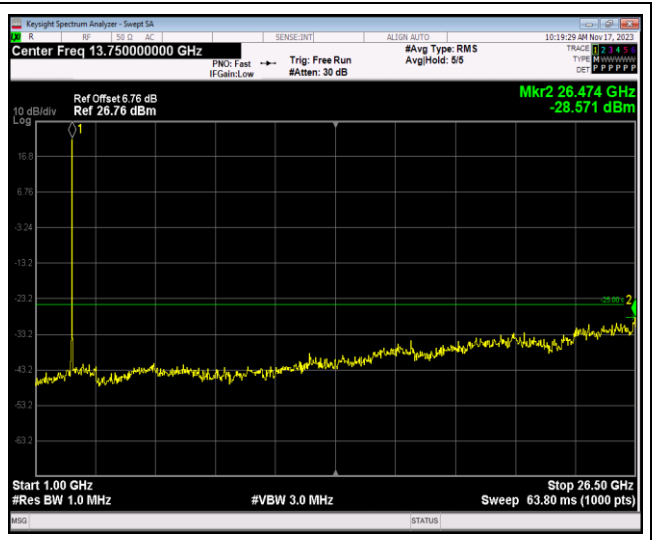
Band7-20MHz-16QAM-20850-1RB#0-Range2:1000~26500MHz
