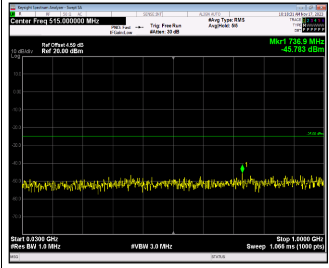
Band7-20MHz-16QAM-21100-1RB#0-Range1:30~1000MHz
