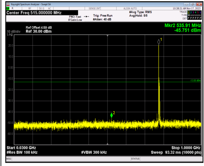
Band13-5MHz-16QAM-23230-1RB#0-Range3:30~1000MHz
