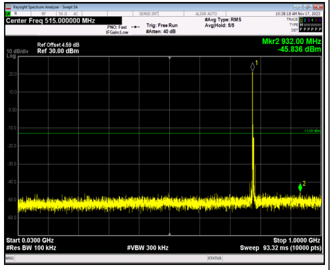
Band13-5MHz-16QAM-23230-1RB#0-Range1:30~1000MHz
