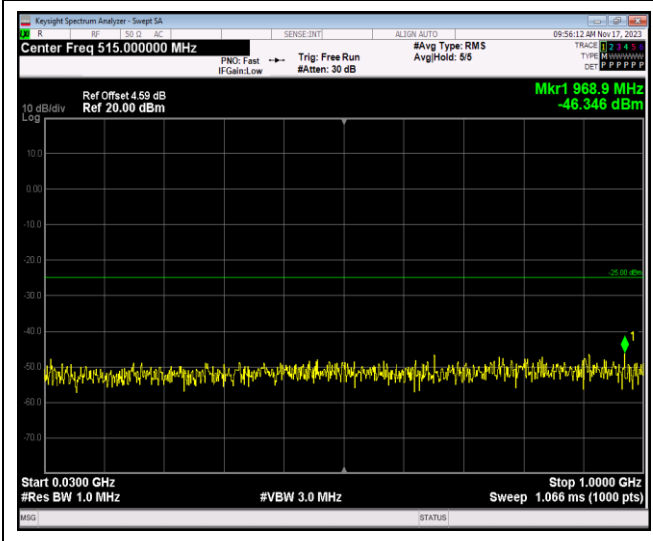
Band7-5MHz-16QAM-21425-1RB#0-Range1:30~100 OMHz
