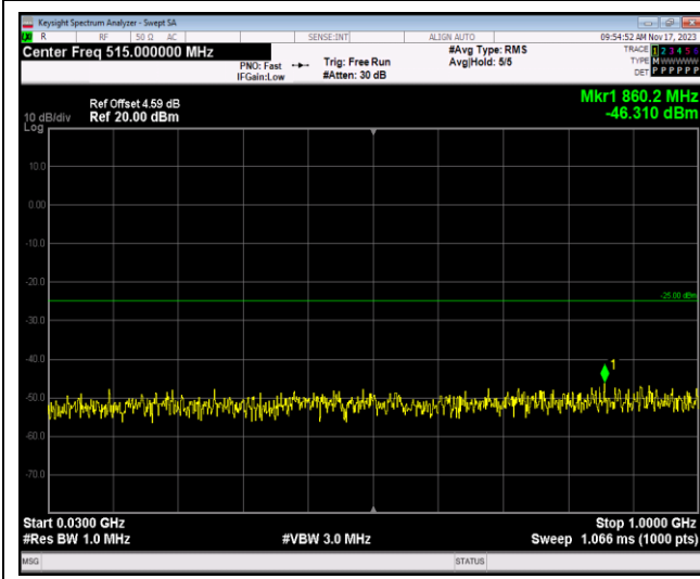
Band7-5MHz-QPSK-20775-1RB#0-Range1:30~1000MHz
