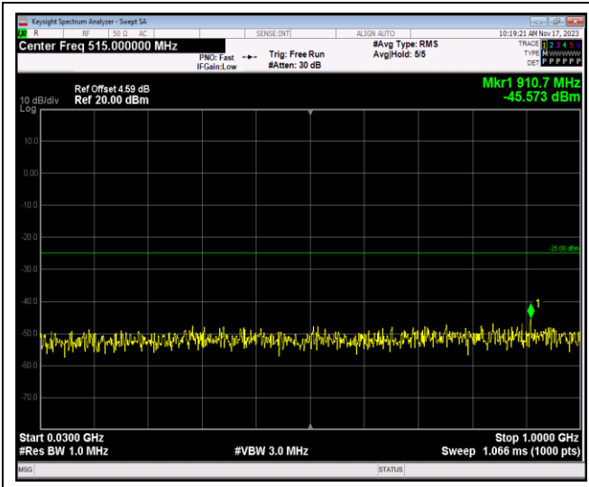
Band7-20MHz-16QAM-20850-1RB#0-Range1:30~1000MHz
