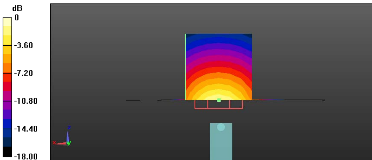
0 dB = 45.4 W/kg = 16.57 dBW/kg
