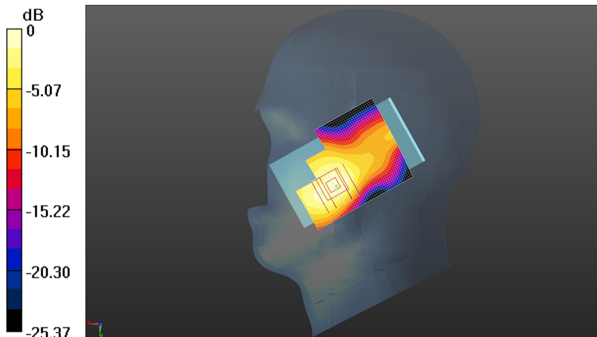
0 dB = 0.120 W/kg = -9.21 dBW/kg
