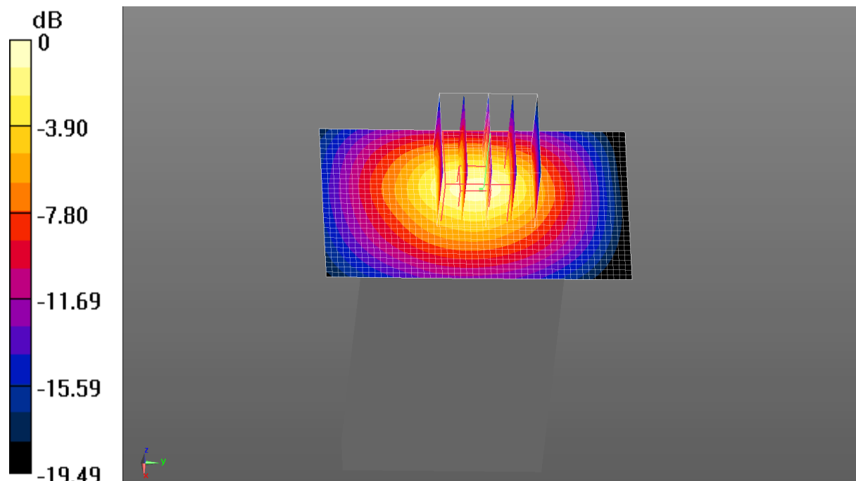
0 dB = 0.390 W/kg = -4.09 dBW/kg
