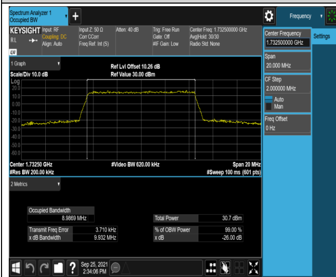
Band4-10MHz-16QAM-20175-50RB#0
