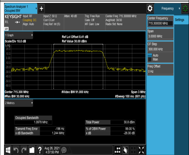
Band12-1.4MHz-QPSK-23173-6RB#0
