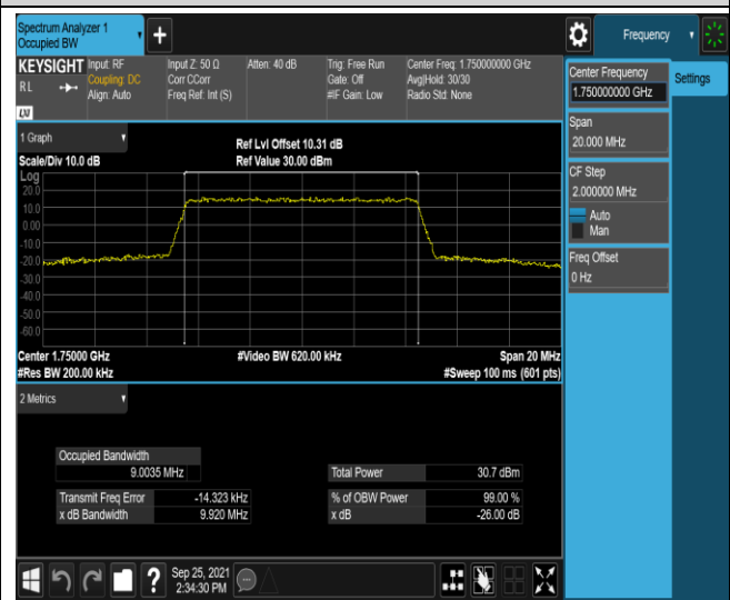
Band4-10MHz-16QAM-20350-50RB#0
