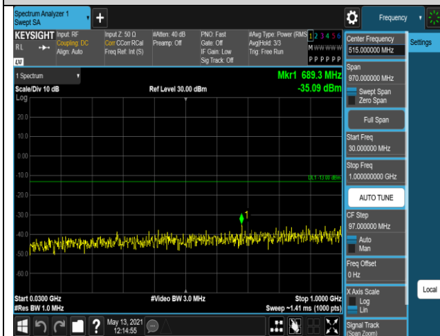
Band4-20MHz-16QAM-20300-1RB#0-Range1:30~1000MHz
