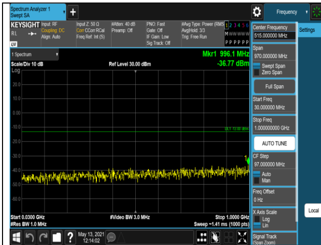
Band4-20MHz-16QAM-20175-1RB#0-Range1:30~1000MHz
