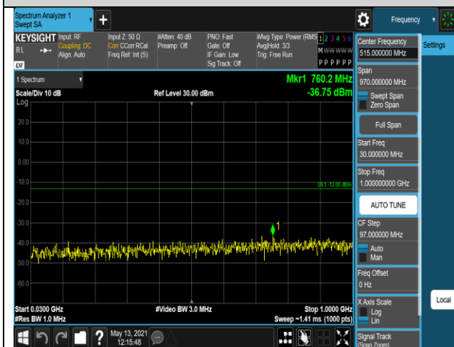
Band5-1.4MHz-QPSK-20407-1RB#0-Range1:30~1000MHz
