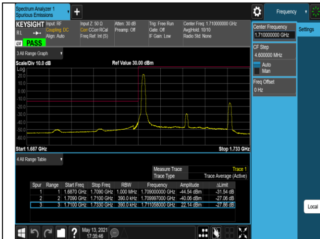
Band66-20MHz-QPSK-132072-100RB#0
