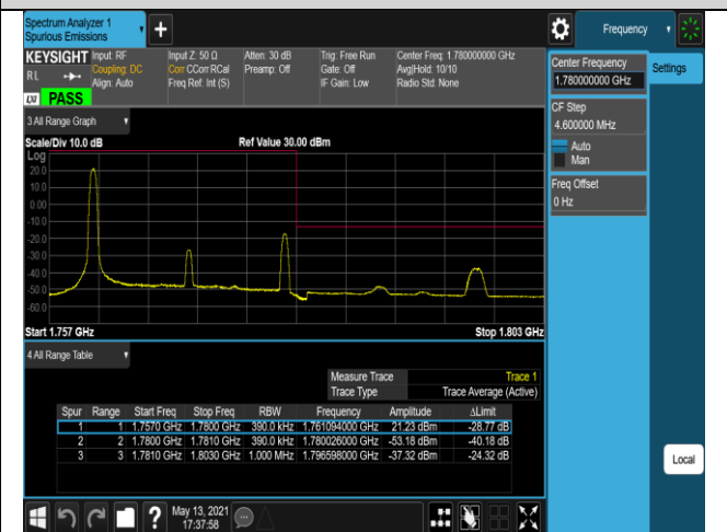
Band66-20MHz-16QAM-132572-100RB#0
