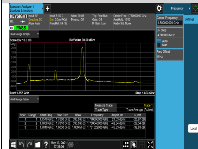
Band66-20MHz-16QAM-132572-1RB#99
