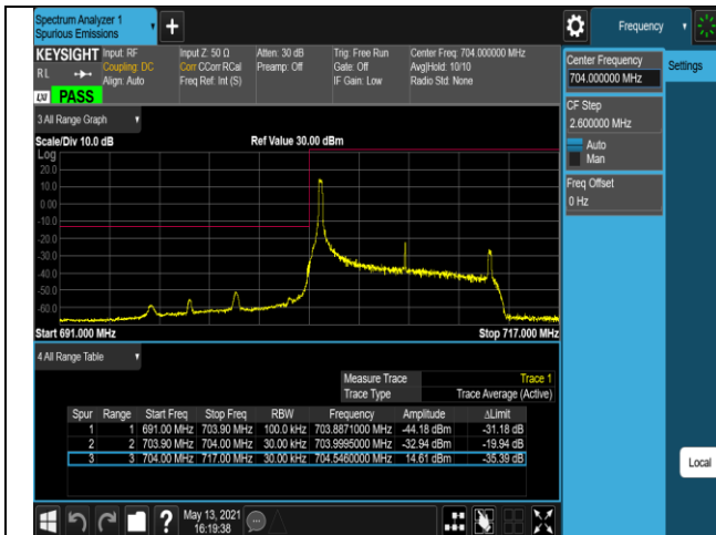
Band17-10MHz-16QAM-23780-50RB#0
