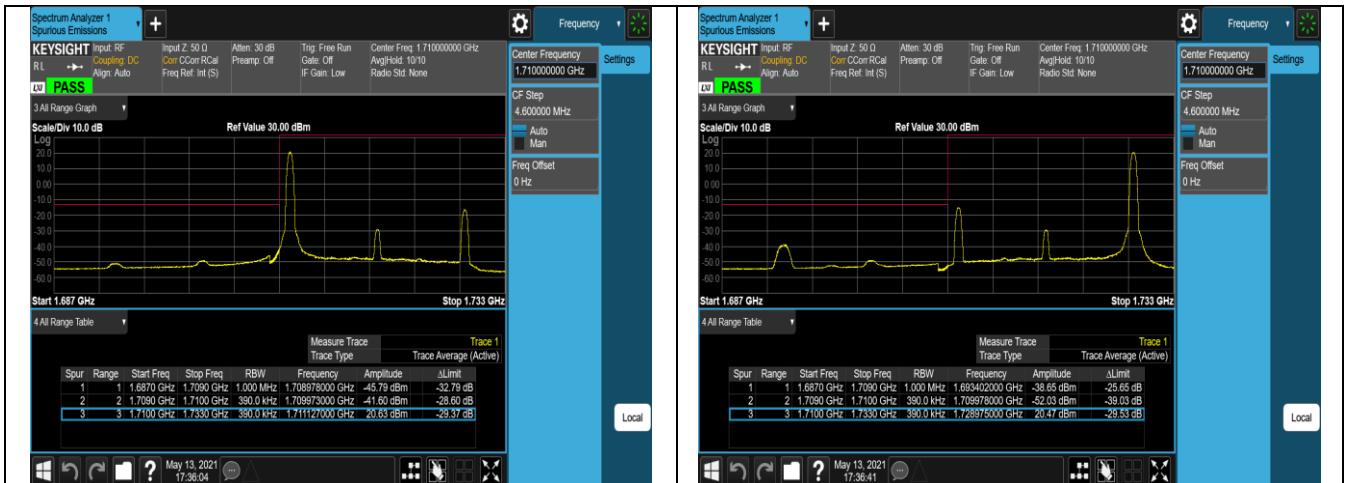
Band66-20MHz-16QAM-132072-100RB#0
