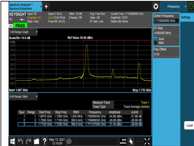
Band4-20MHz-16QAM-20050-100RB#0
