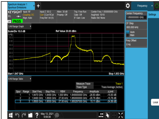
Band2-1.4MHz-16QAM-18607-6RB#0
