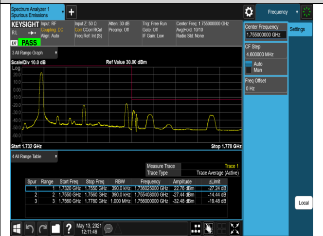
Band4-20MHz-QPSK-20300-100RB#0
