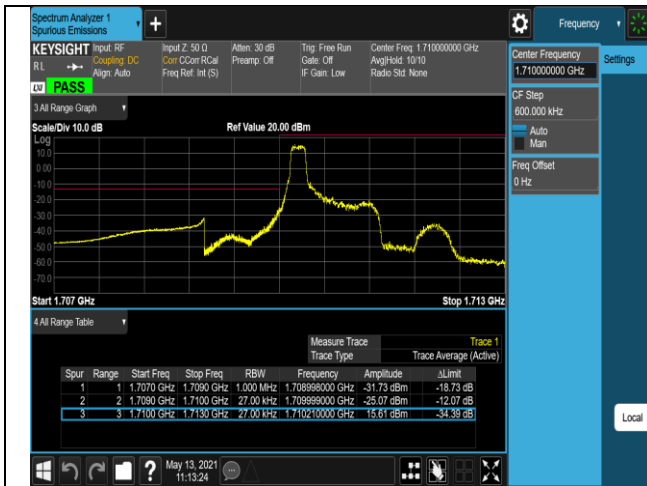
Band4-1.4MHz-16QAM-19957-6RB#0
