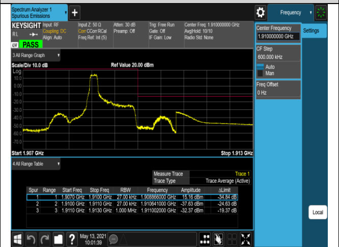
Band2-1.4MHz-16QAM-19193-6RB#0
