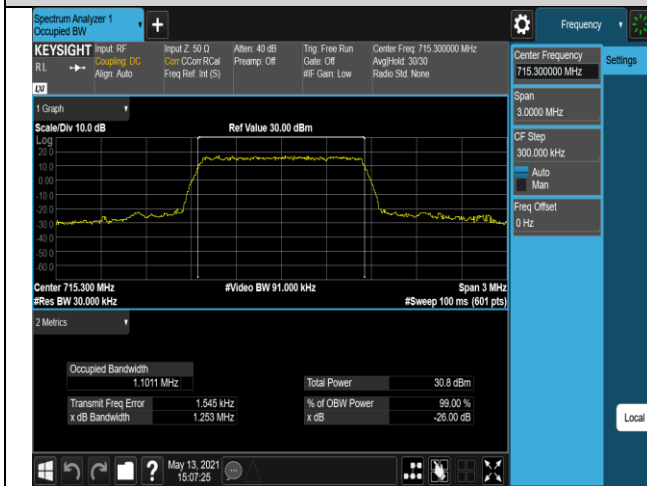
Band12-1.4MHz-16QAM-23095-6RB#0
