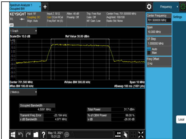
Band12-5MHz-QPSK-23155-25RB#0
