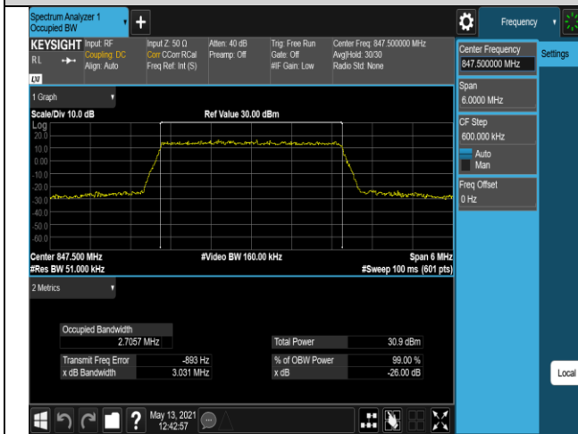
Band5-3MHz-16QAM-20525-15RB#0
