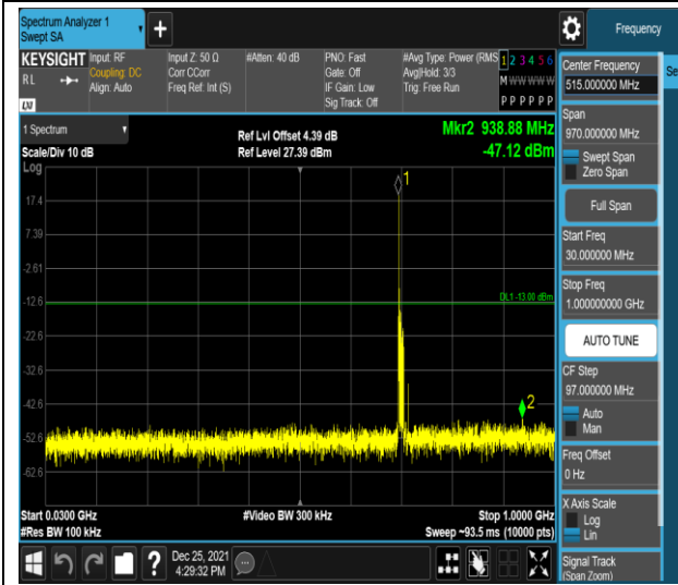
Band12-10MHz-16QAM-23130-1RB#0-Range1:30 ~1000MHz
