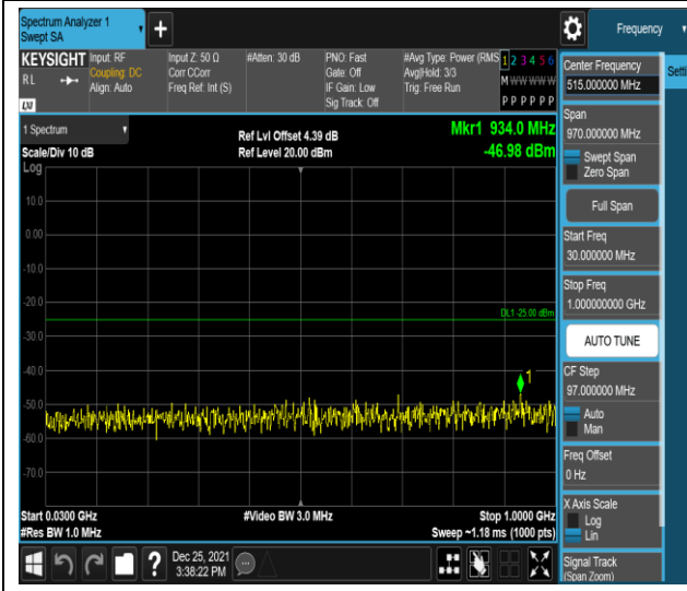
Band7-20MHz-QPSK-21350-1RB#0-Range1:30~1000MHz
