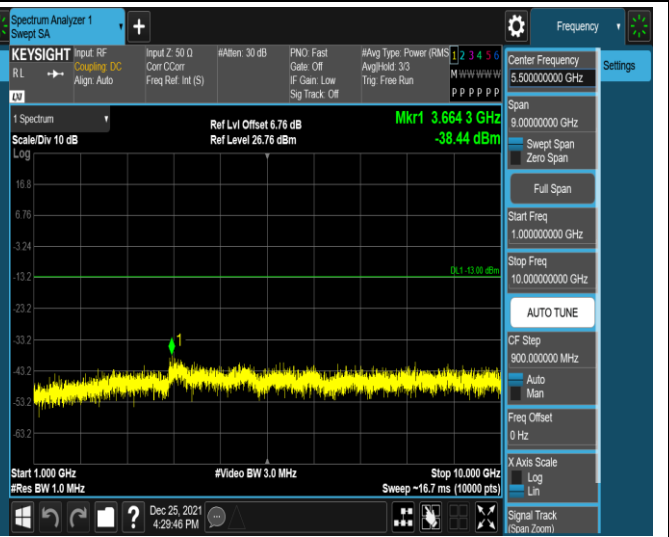
Band12-10MHz-16QAM-23130-1RB#0-Range2:1000~ 10000MHz
