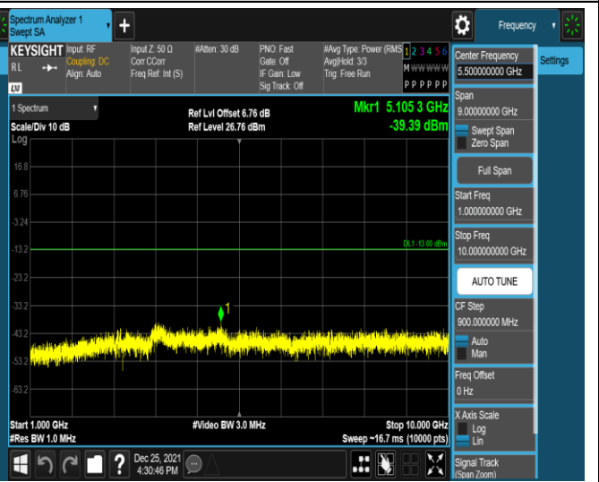
Band12-10MHz-16QAM-23130-1RB#0-Range2:1000~ 10000MHz
