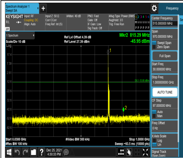
Band12-10MHz-16QAM-23130-1RB#0-Range1:30 ~1000MHz
