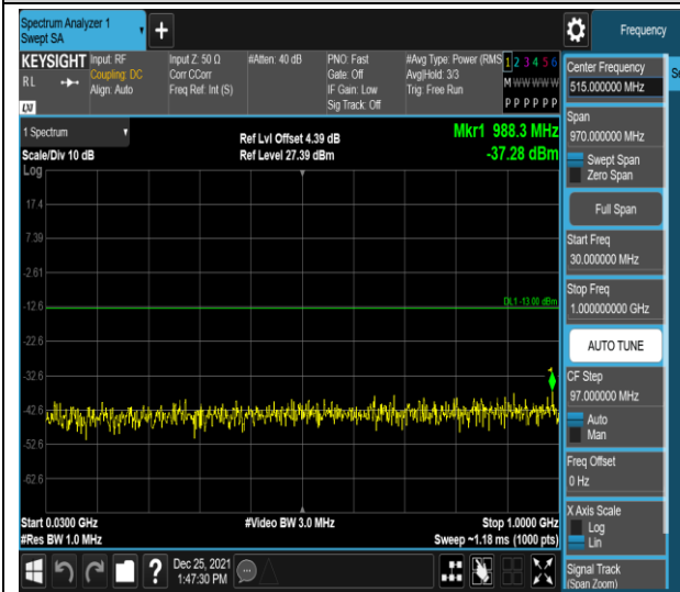
Band4-20MHz-QPSK-20175-1RB#0-Range1:30~1000MHz
