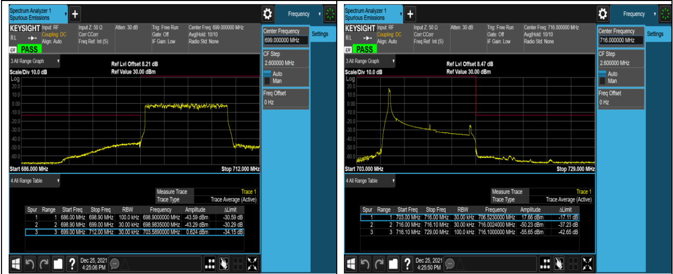
Band12-10MHz-QPSK-23130-1RB#49
