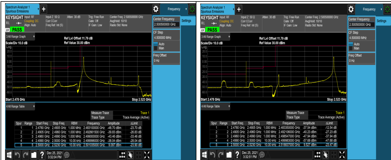
Band7-20MHz-16QAM-20850-100RB#0
