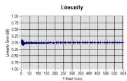
Linearity: +/-1.97% (+/-0.09dB)
