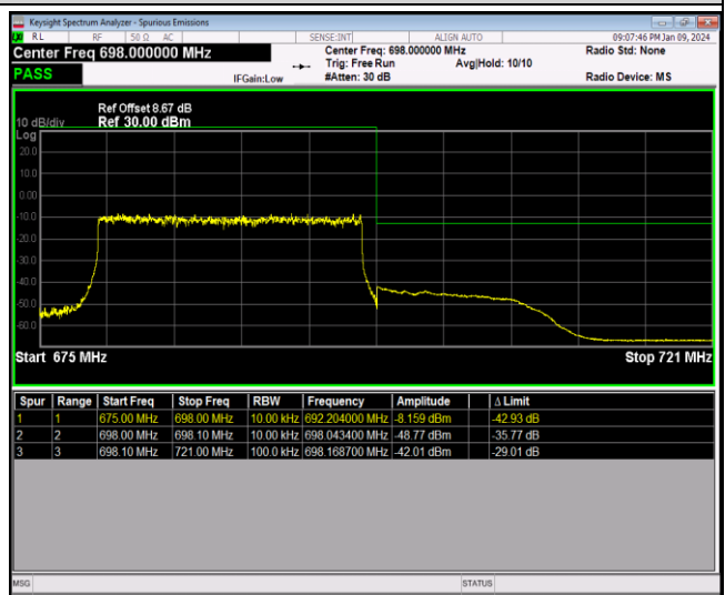
Band71-20MHz-16QAM-133222-1RB#99
