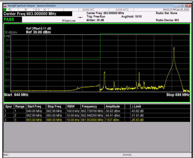
Band71-20MHz-64QAM-133372-1RB#0
