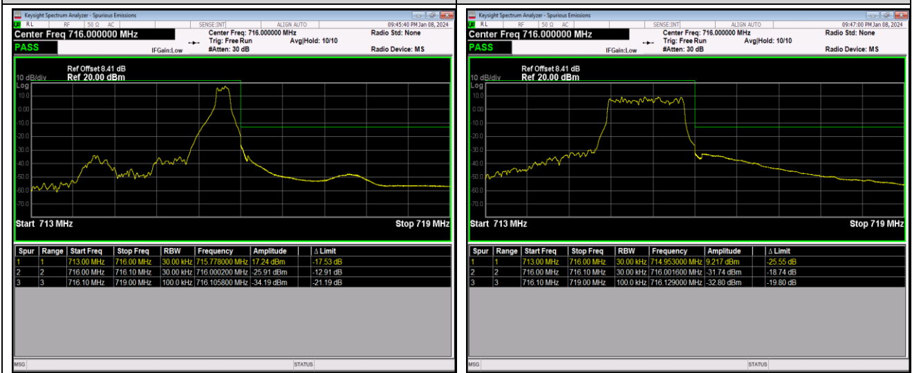
Band12-1.4MHz-64QAM-23017-1RB#0
