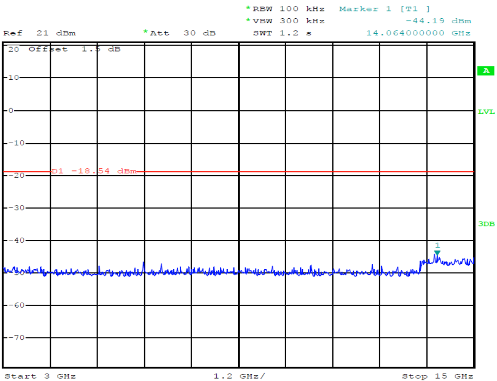
(Plot 4.6.3 C1: Channel 11: 2462MHz @ 802.11n(20MHz))
