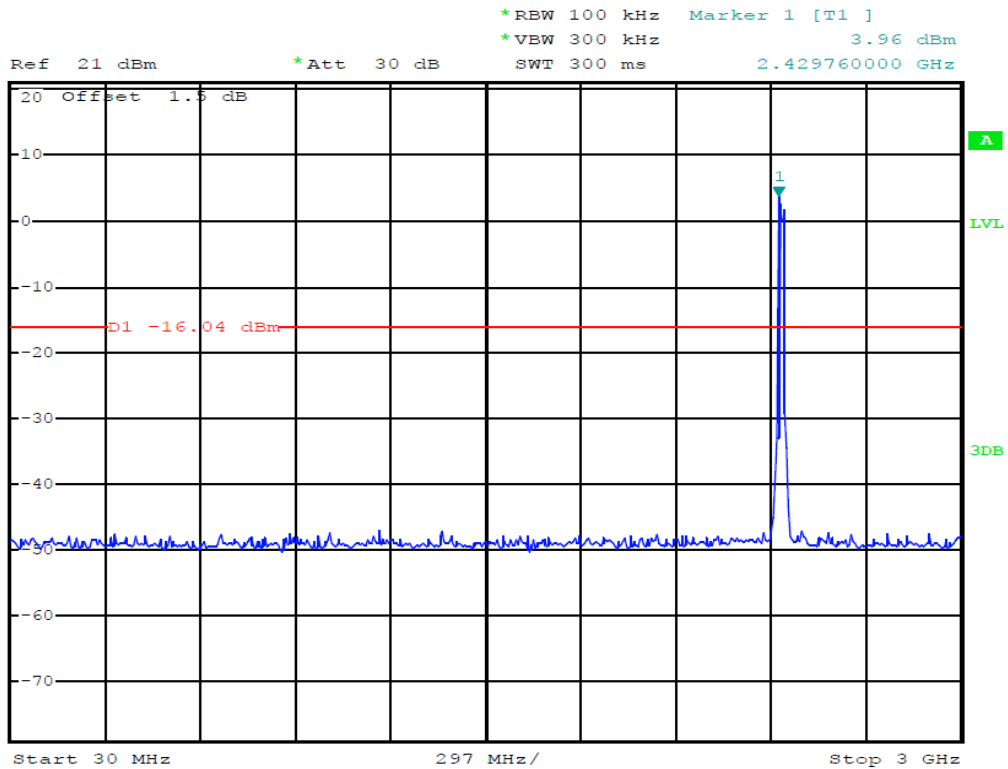
(Plot 4.6.2 A3: Channel 1: 2412MHz @ 802.11g)
