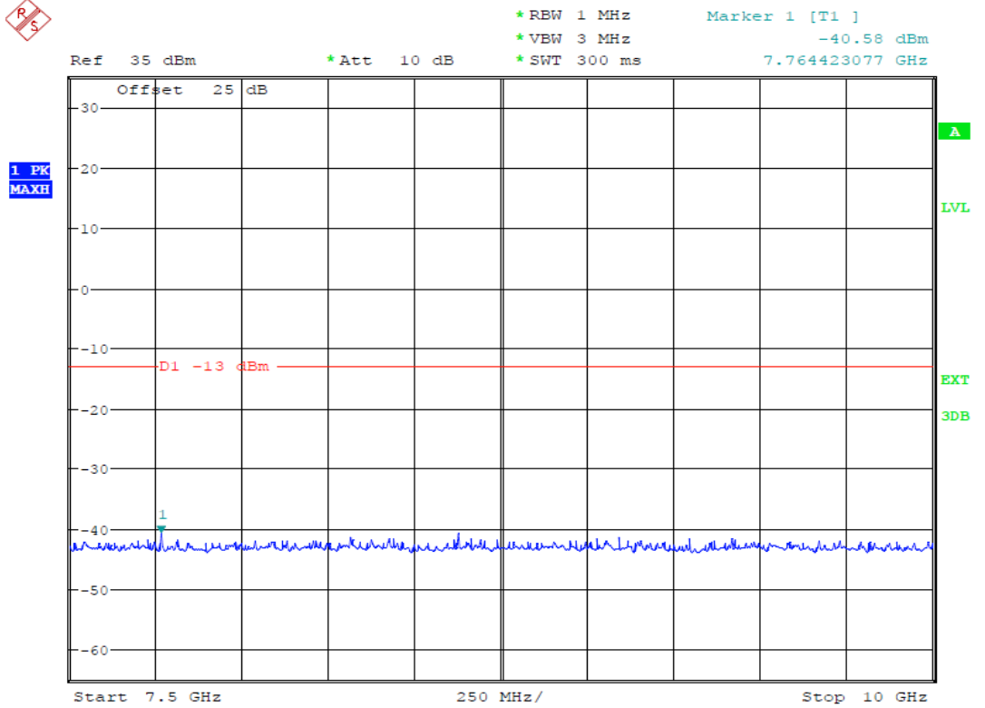
(Plot 4.7.4 A3: Idle @ GSM850)
