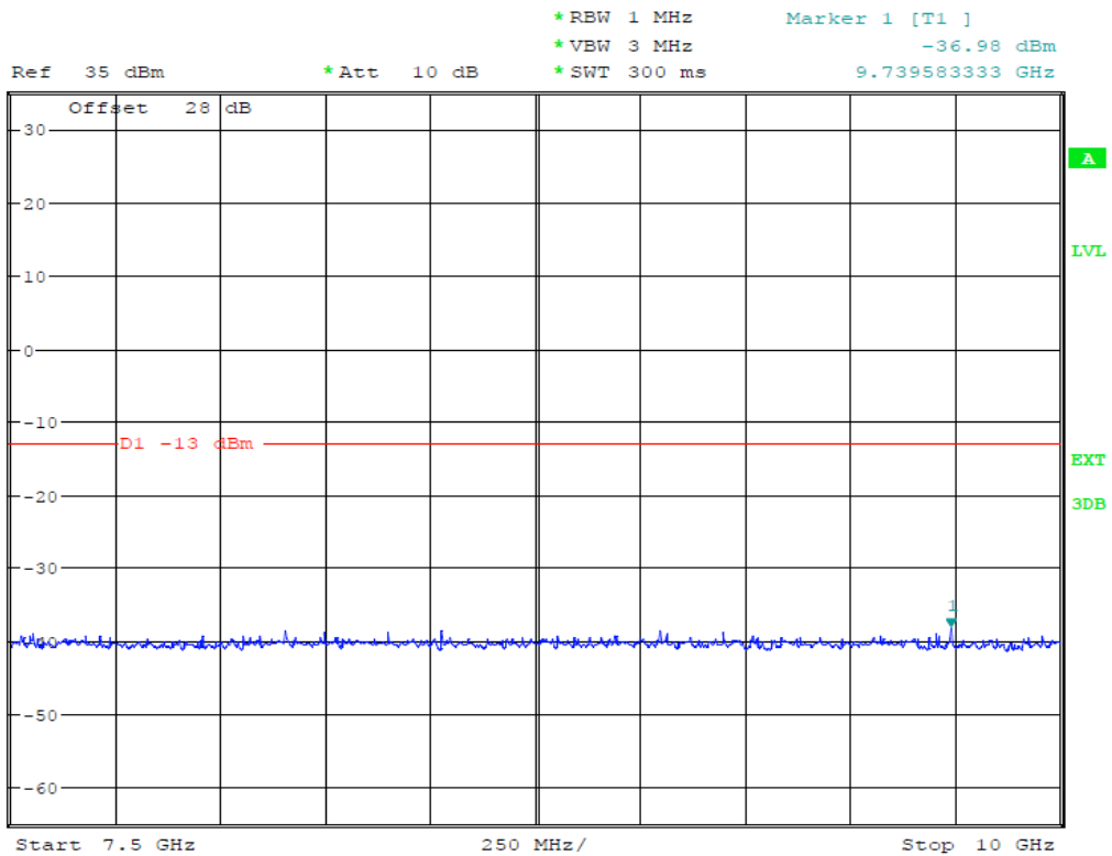
(Plot 4.7.7 A3: Channel 810: 1909.80MHz @ Traffic @ PCS1900)
