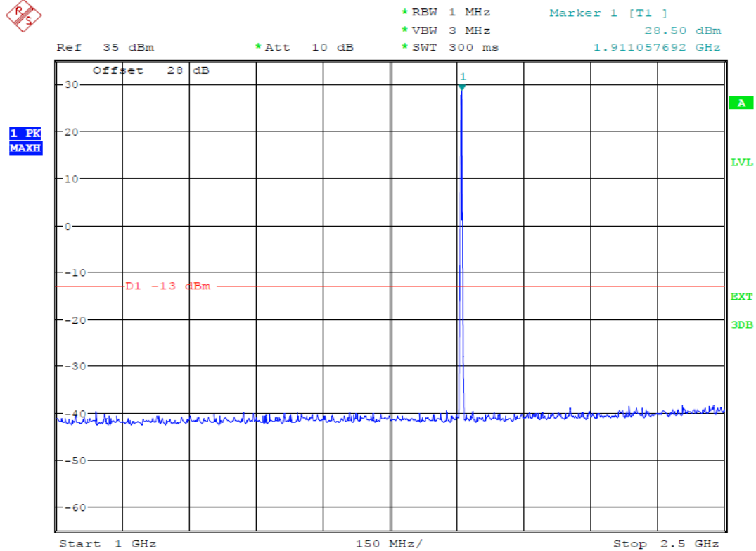
(Plot 4.7.7 A1: Channel 810: 1909.80MHz @ Traffic @ PCS1900)
