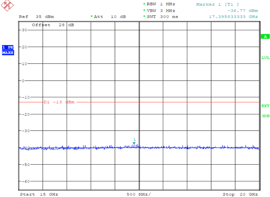
(Plot 4.7.7 A5: Channel 810: 1909.80MHz @ Traffic @ PCS1900)
