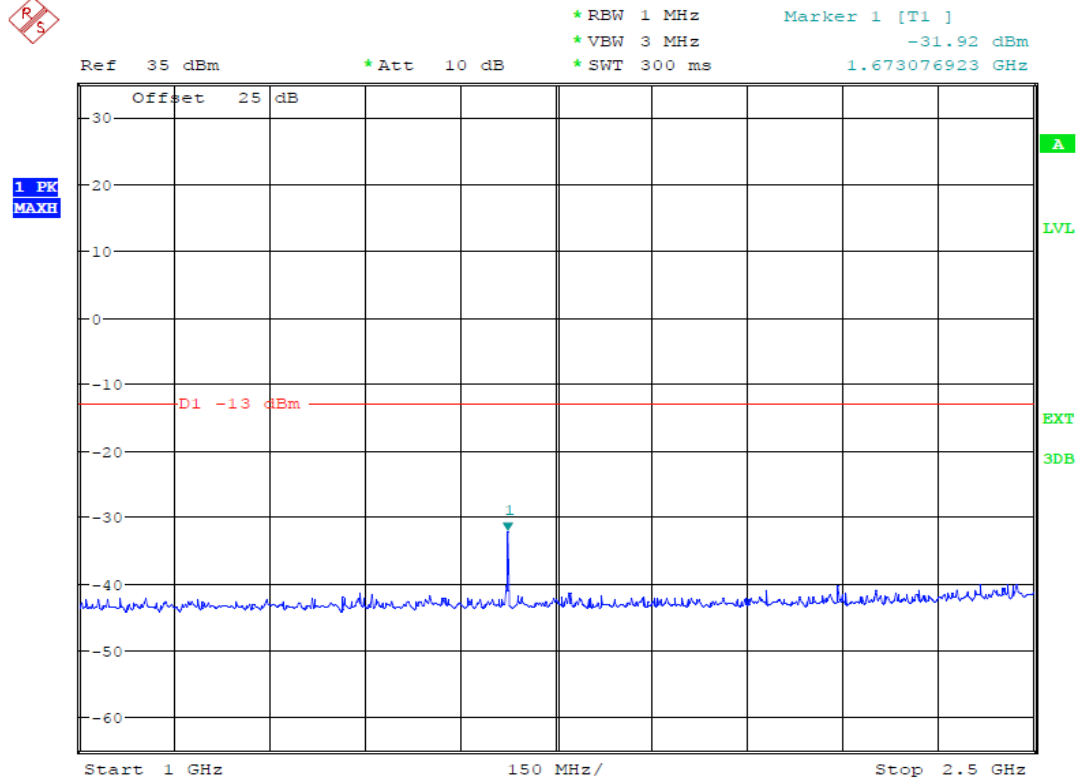
(Plot 4.7.2 A1: Channel 190: 836.60MHz @ Traffic @ GSM850)
