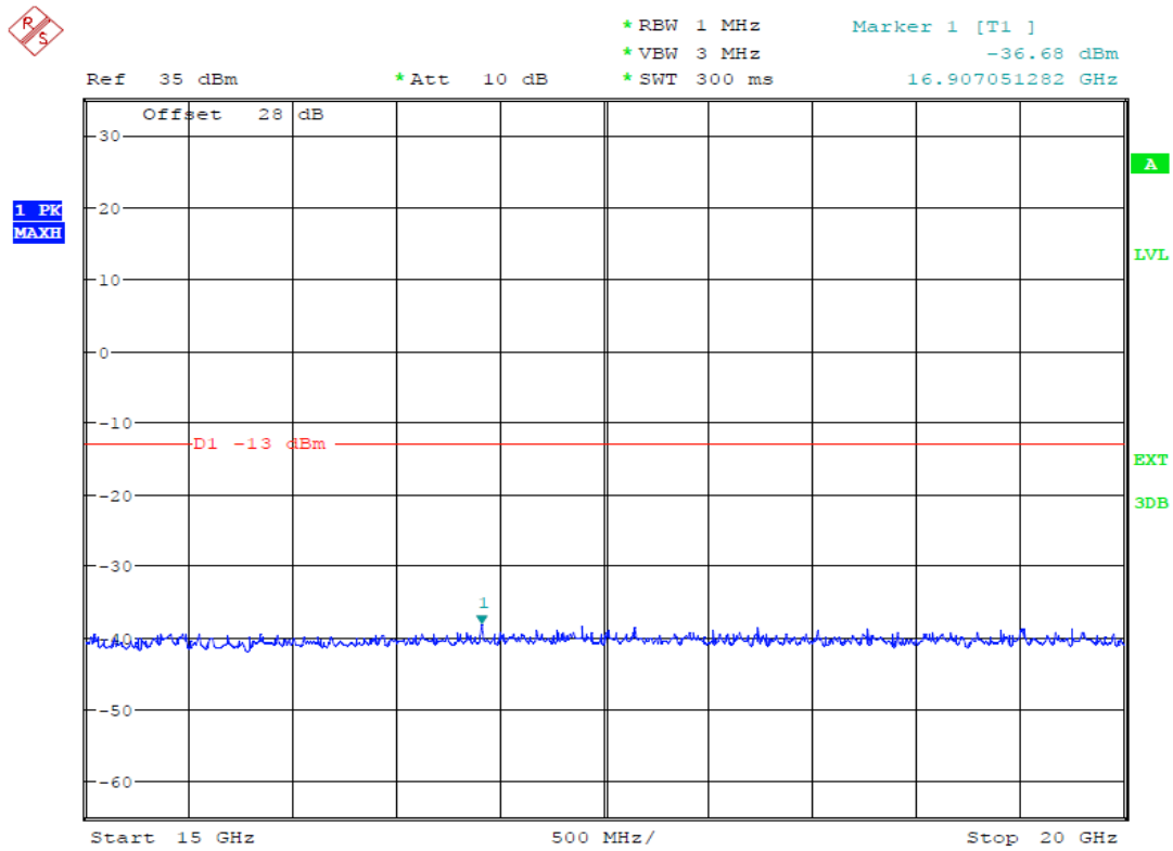
(Plot 4.7.8 A5: Idle @ PCS1900)
