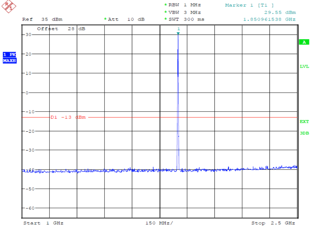
(Plot 4.7.5 A1: Channel 512: 1850.20MHz @ Traffic @ PCS1900)
