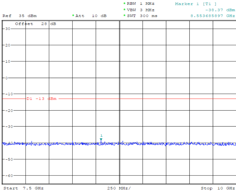
(Plot 4.7.6 A3: Channel 661: 1880.00MHz @ Traffic @ PCS1900)
