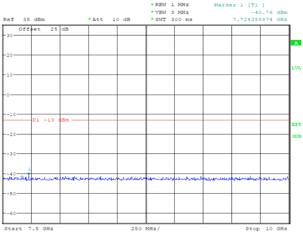
(Plot 4.7.3 A3: Channel 251: 848.80MHz @ Traffic @ GSM850)
