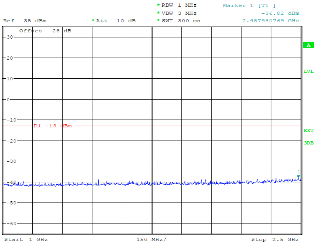
(Plot 4.7.8 A1: Idle @ PCS1900)
