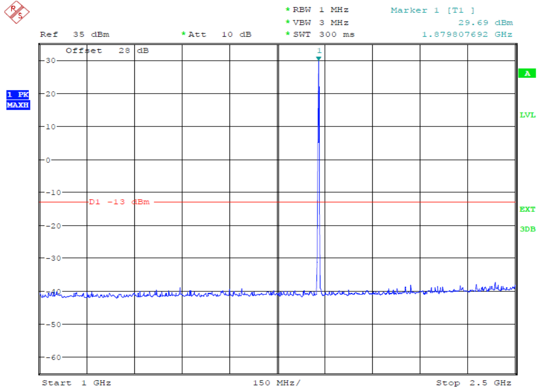
(Plot 4.7.6 A1: Channel 661: 1880.00MHz @ Traffic @ PCS1900)
