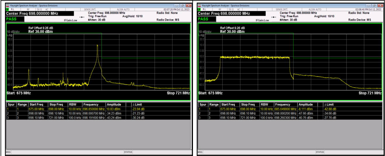
Band71-20MHz-64QAM-133222-1RB#0
