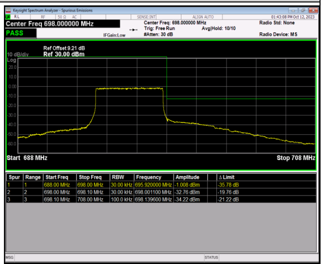
Band71-5MHz-64QAM-133147-1RB#24
