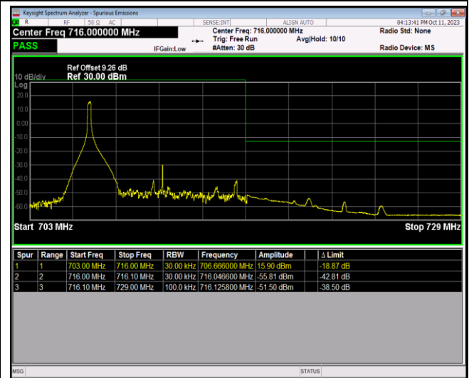
Band17-10MHz-16QAM-23800-50RB#0
