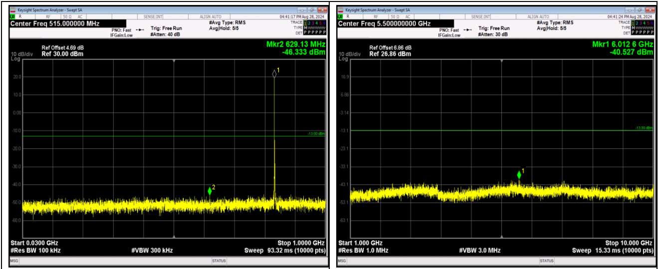
Band5-1.4MHz-16QAM-20643-1RB#0-Range1:30~1000MHz
