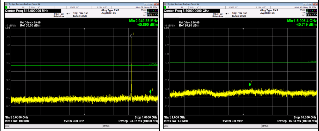
Band5-1.4MHz-64QAM-20407-1RB#0-Range1:30~1000MHz
