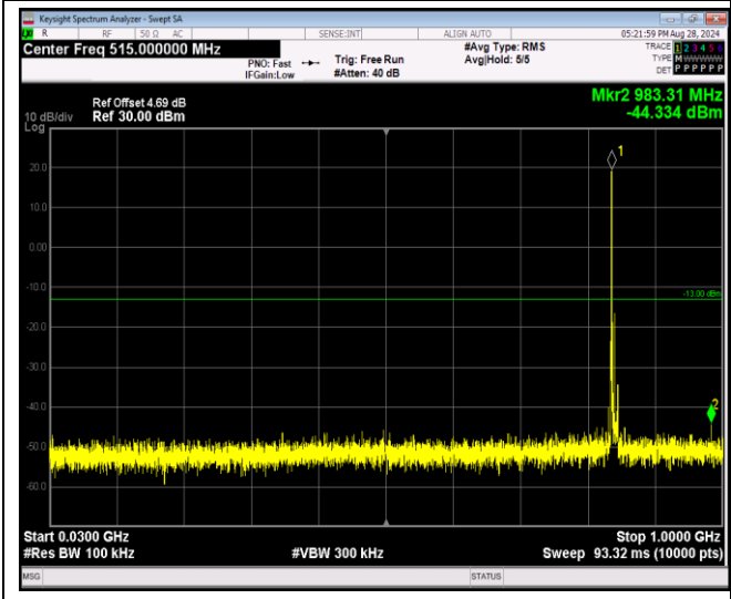
Band5-10MHz-QPSK-20600-1RB#0-Range1:30~100 OMHz
