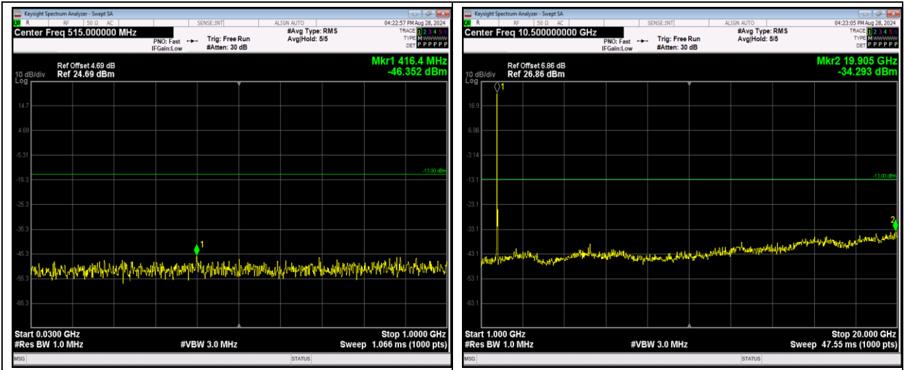
Band5-1.4MHz-QPSK-20407-1RB#0-Range1:30~1000MHz
