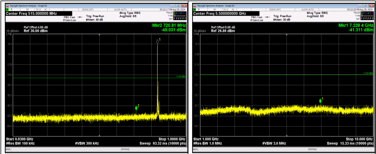
Band5-10MHz-64QAM-20450-1RB#0-Range1:30~1000MHz
