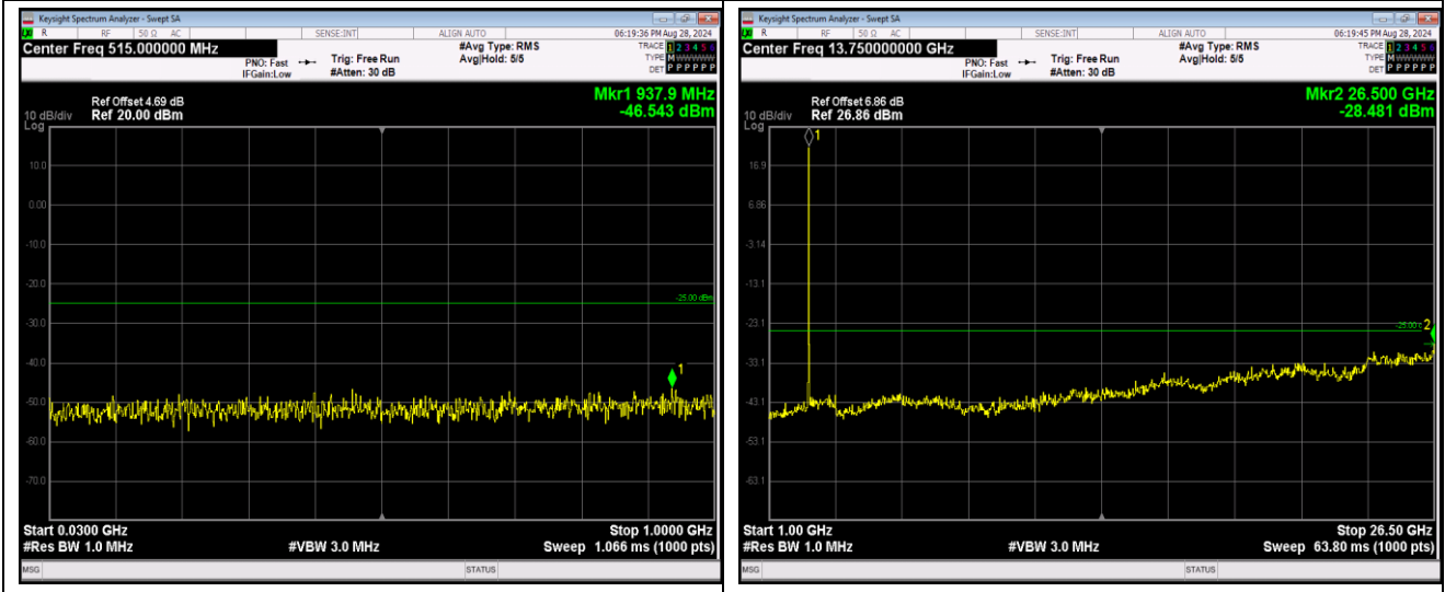
Band7-20MHz-16QAM-21100-1RB#0-Range1:30~1000MHz
