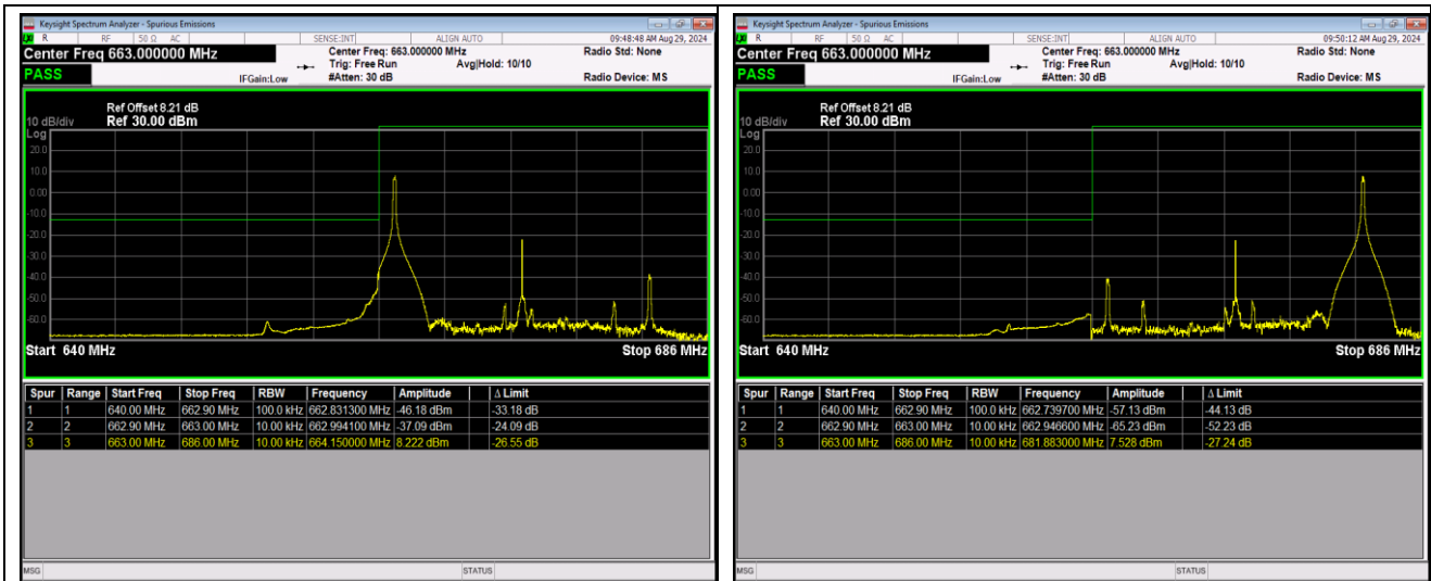
Band71-20MHz-64QAM-133222-100RB#0
