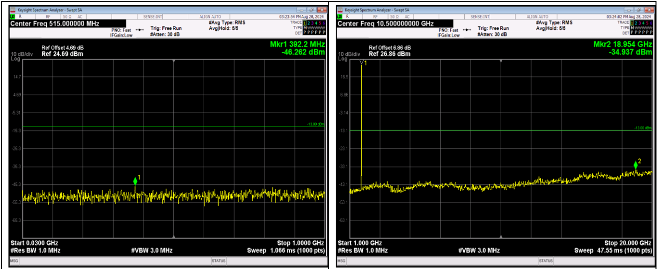
Band4-1.4MHz-16QAM-19957-1RB#0-Range1:30~1000MHz
