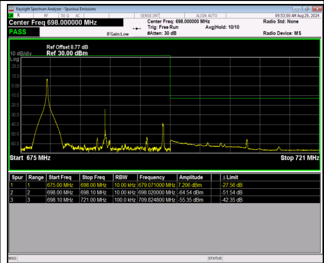
Band71-20MHz-64QAM-133372-100RB#0
