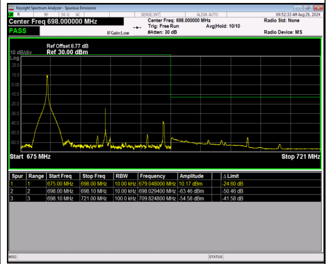
Band71-20MHz-16QAM-133372-100RB#0
