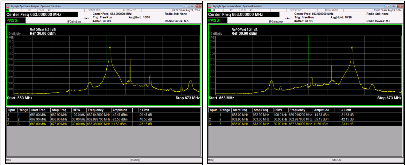
Band71-5MHz-64QAM-133147-25RB#0 Band71-5MHz-64QAM-133447-1RB#0
