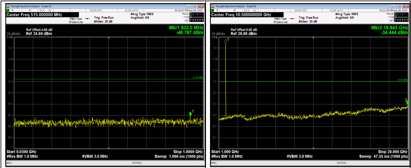
Band4-20MHz-16QAM-20175-1RB#0-Range1:30~1000MHz
