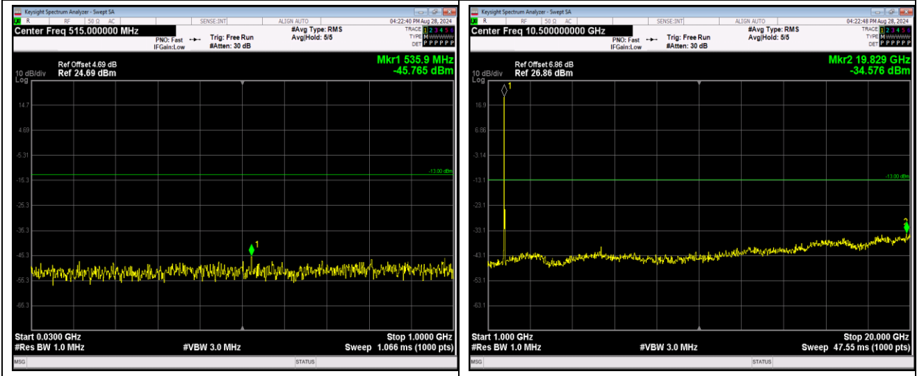
Band4-20MHz-16QAM-20300-1RB#0-Range1:30~1000MHz
