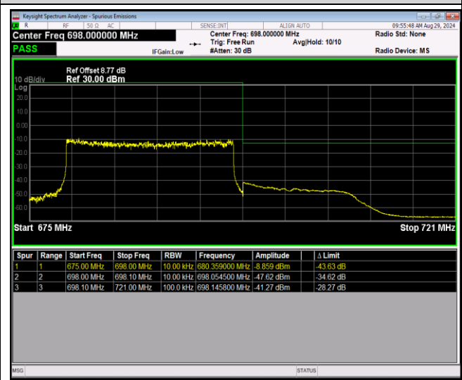
Band71-20MHz-64QAM-133372-100RB#0
