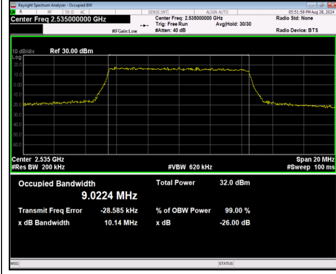
Band7-10MHz-16QAM-20800-50RB#0
