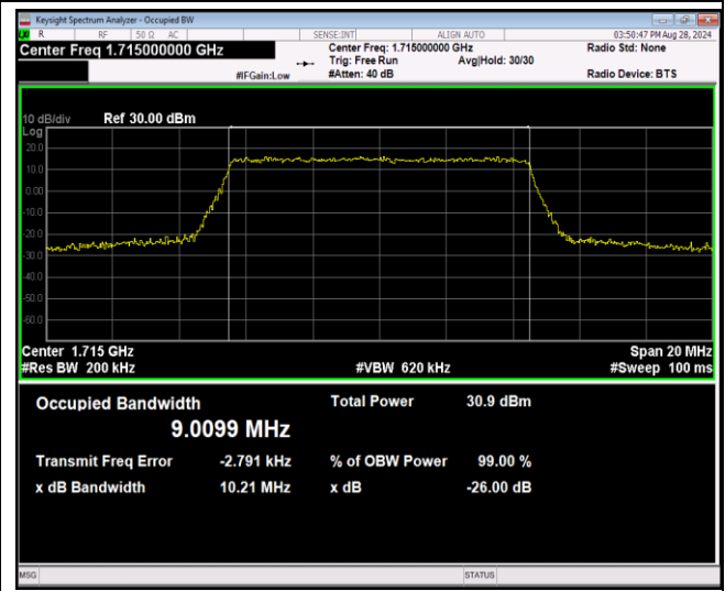
Band4-10MHz-QPSK-20350-50RB#0
