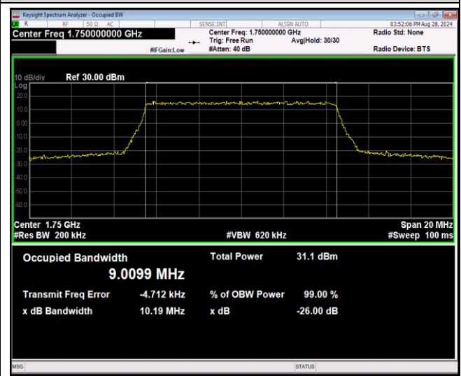
Band4-10MHz-16QAM-20175-50RB#0
