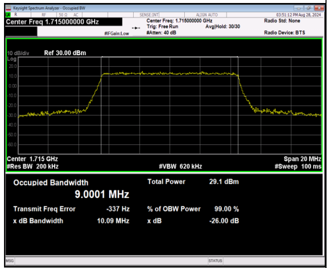
Band4-10MHz-64QAM-20350-50RB#0
