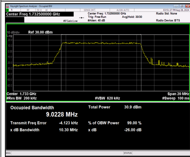
Band4-10MHz-16QAM-20000-50RB#0
