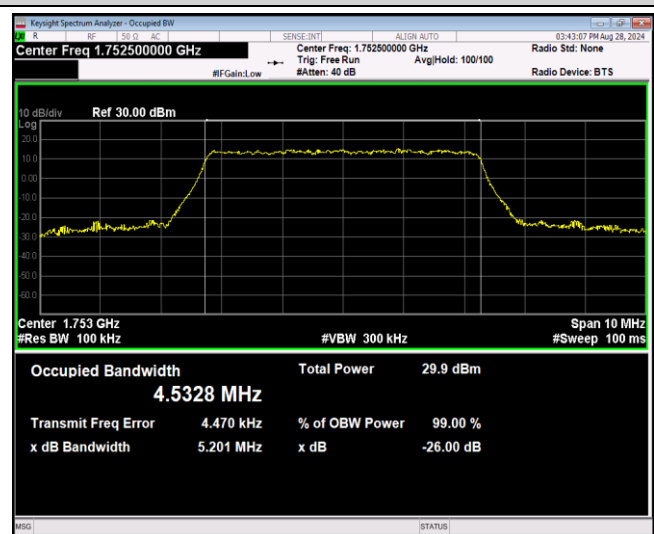
Band4-5MHz-64QAM-20175-25RB#0
