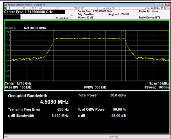
Band4-5MHz-16QAM-20375-25RB#0
