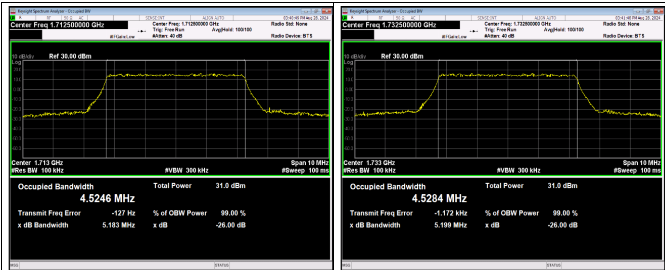
Band4-5MHz-QPSK-20375-25RB#0
