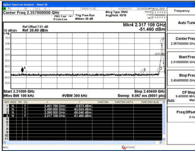
Channel 0 / 2402 MHz
