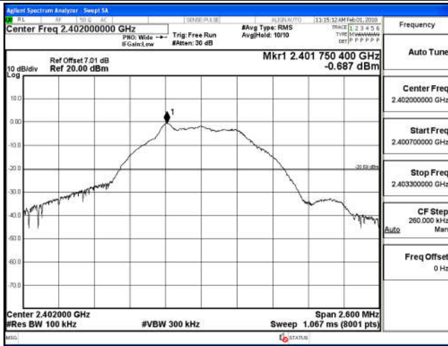
2400.5 MHz – 2403.5 MHz
