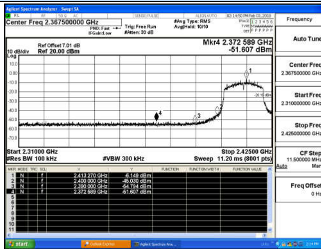
Channel 1 / 2412 MHz
