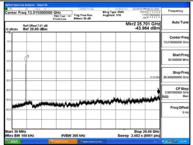
30 MHz – 26 GHz
