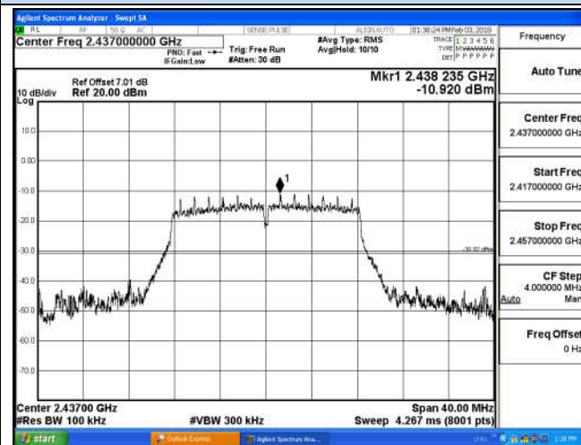
2422 MHz – 2452 MHz
