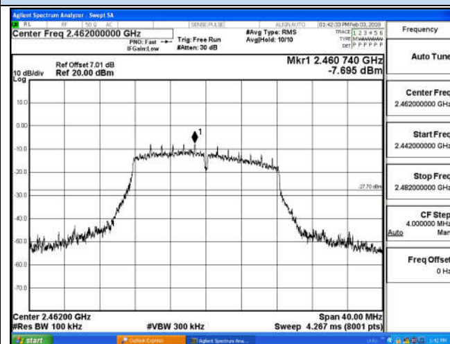
2447 MHz – 2477 MHz
