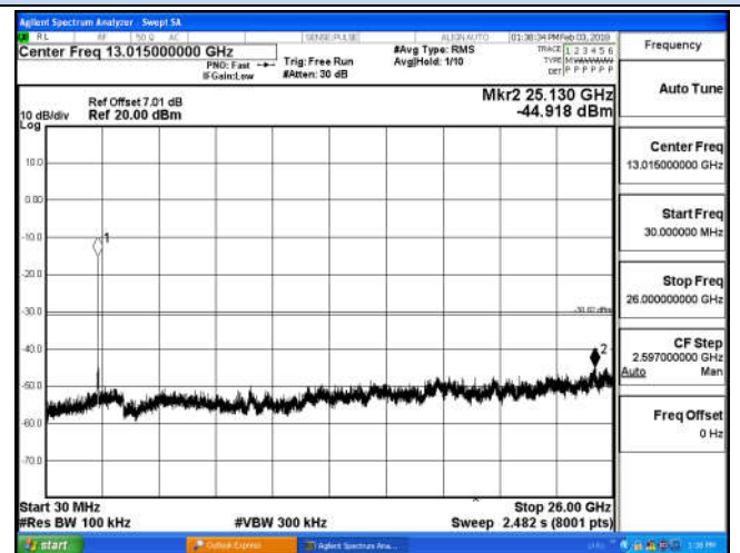
30 MHz – 26 GHz
