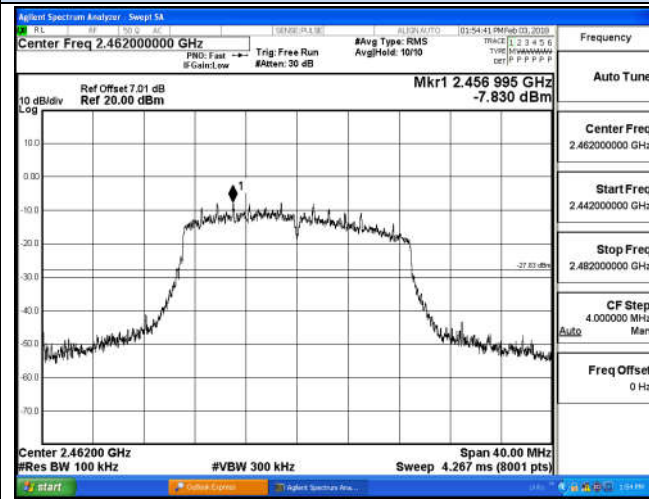
2447 MHz – 2477 MHz
