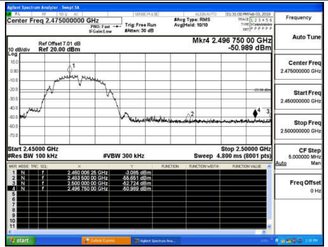
Channel 11 / 2462 MHz
