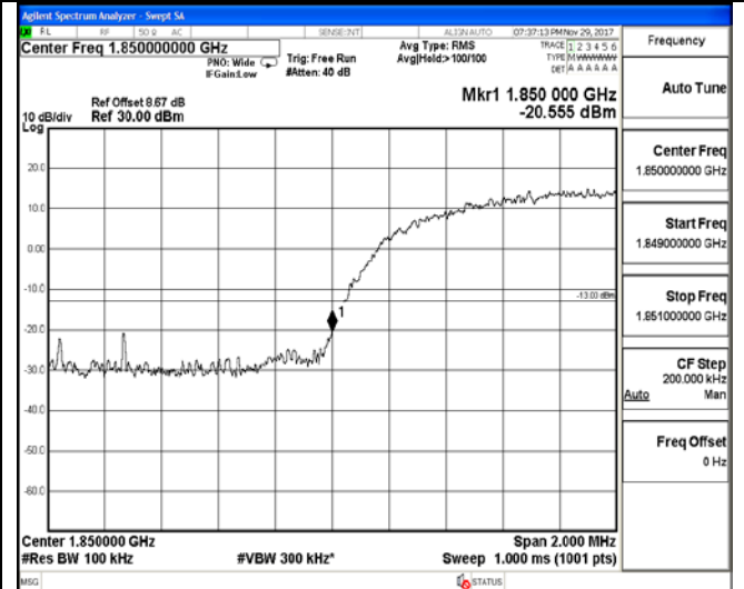
Channel 9262 / 1852.4 MHz
