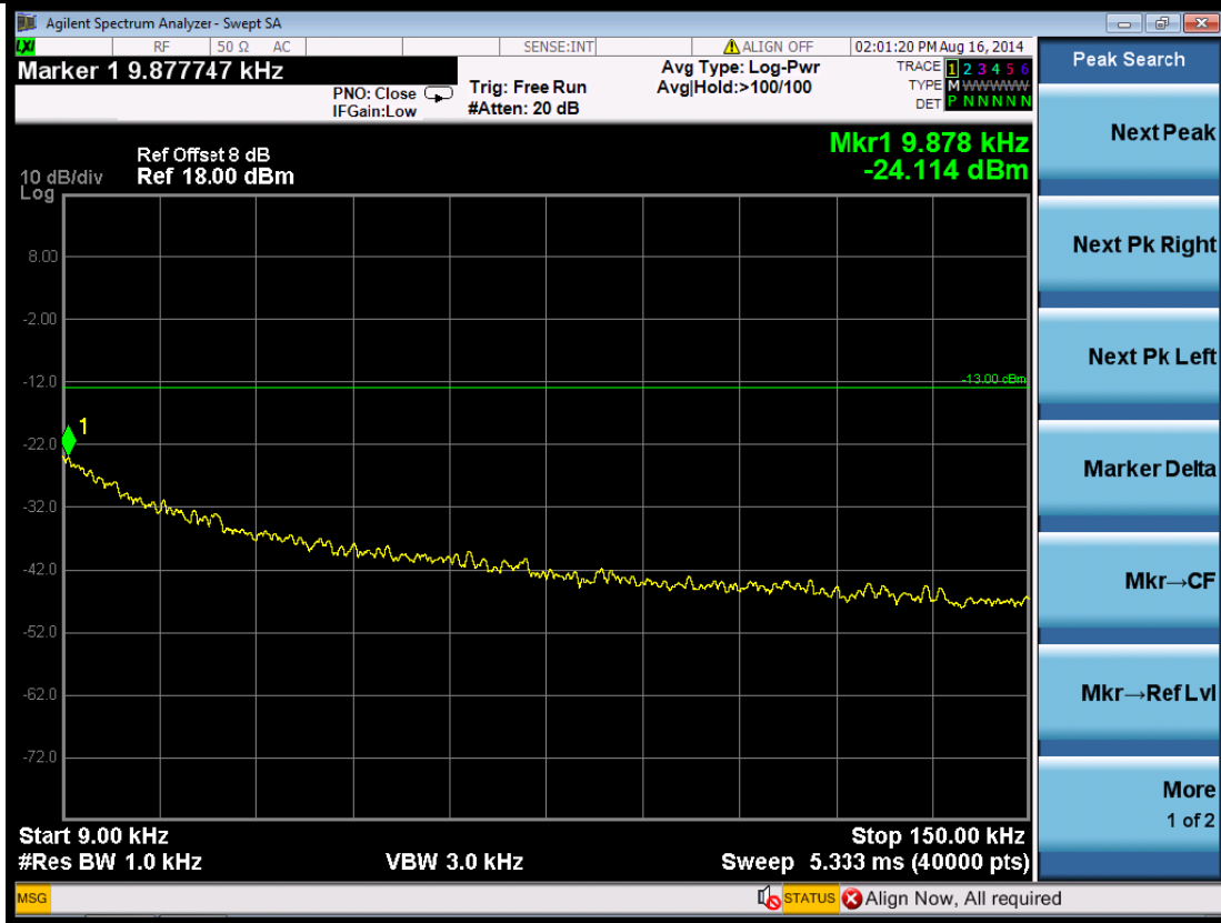
(Plot 5.5.3 D1: Idle WCDMA Band IV)
