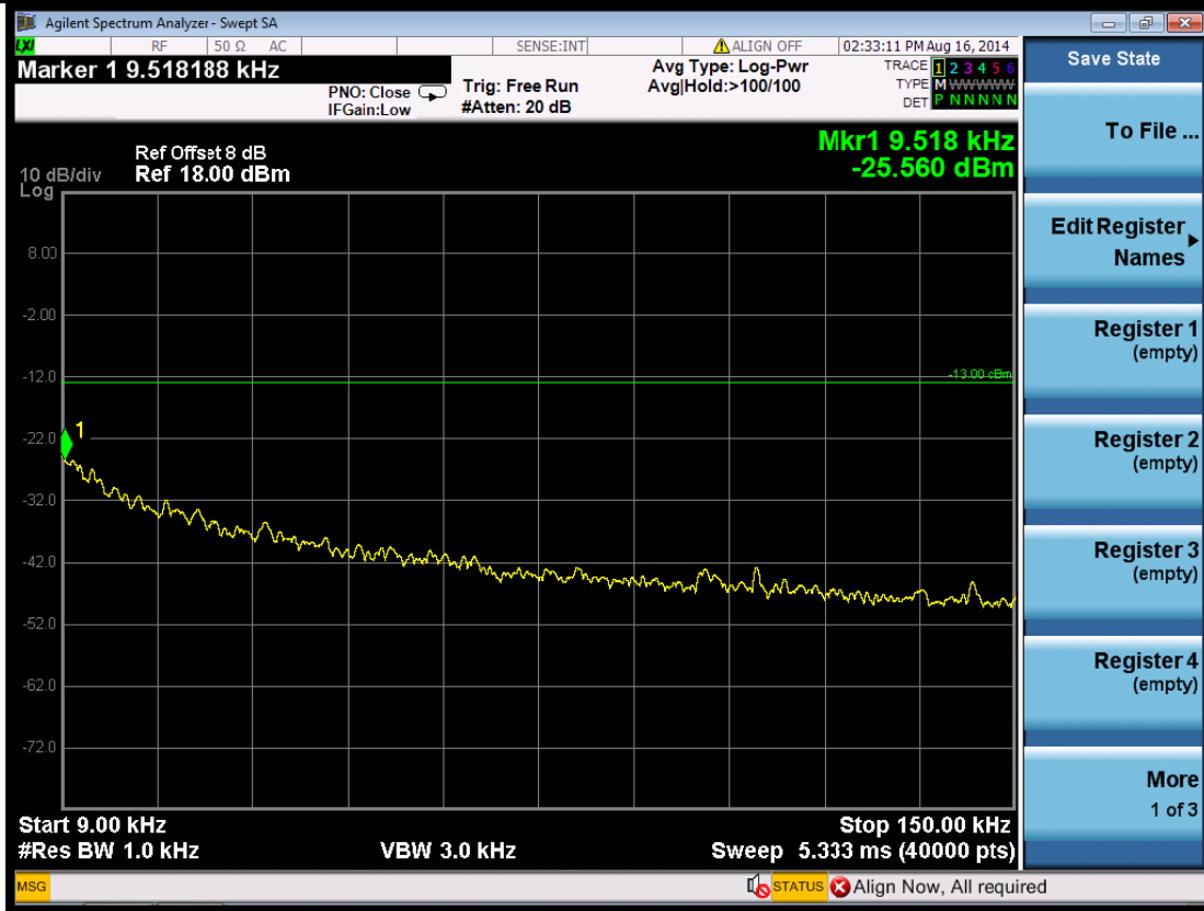
(Plot 5.5.1 A1: Channel 9262: 1852.4MHz @ Traffic WCDMA Band II)
