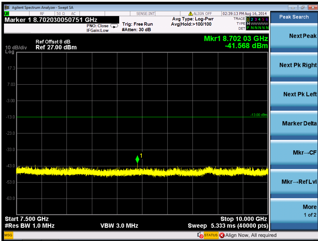
(Plot 5.5.1 A6: Channel 9262: 1852.4MHz @ Traffic WCDMA Band II)
