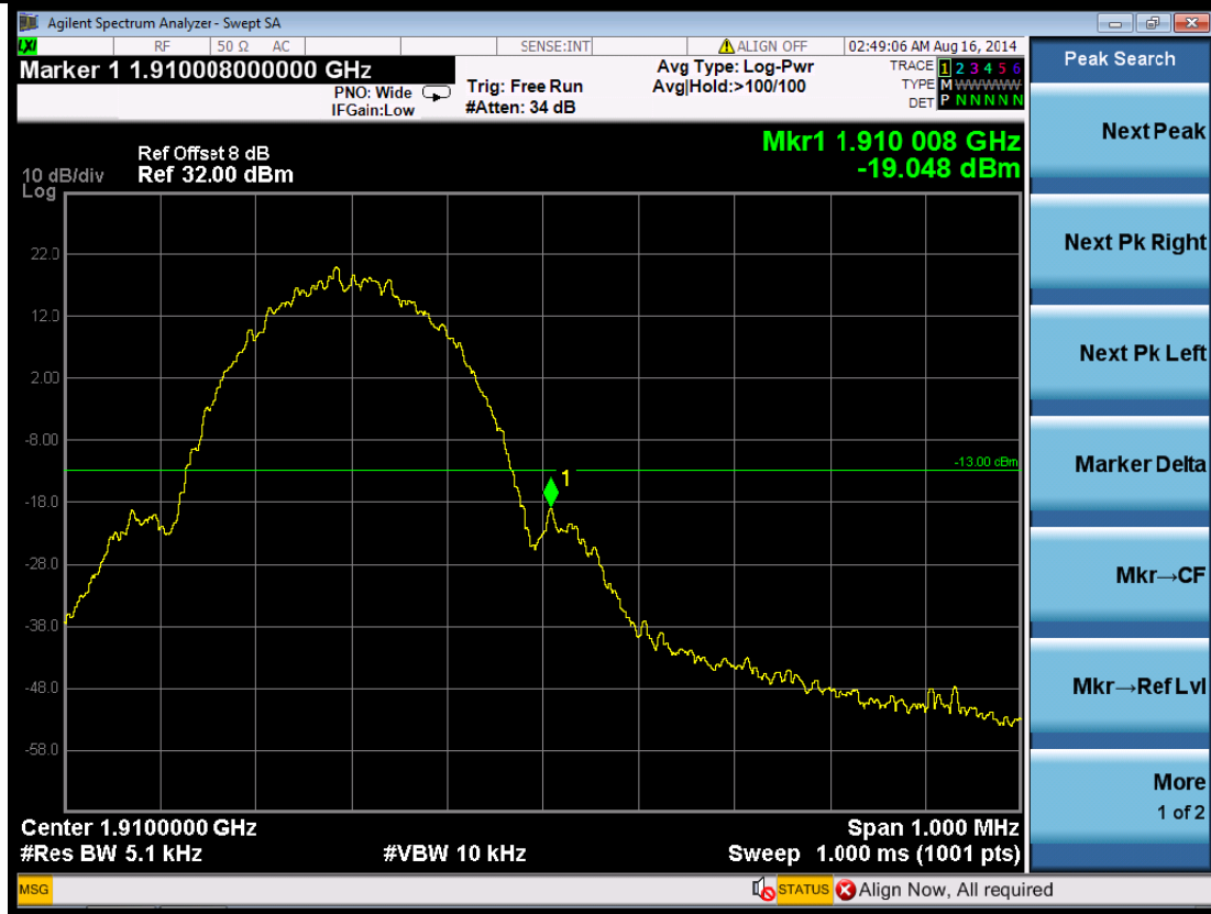
(Plot 5.4.3 B: Channel 810: 1909.80MHz @ GPRS1900)
