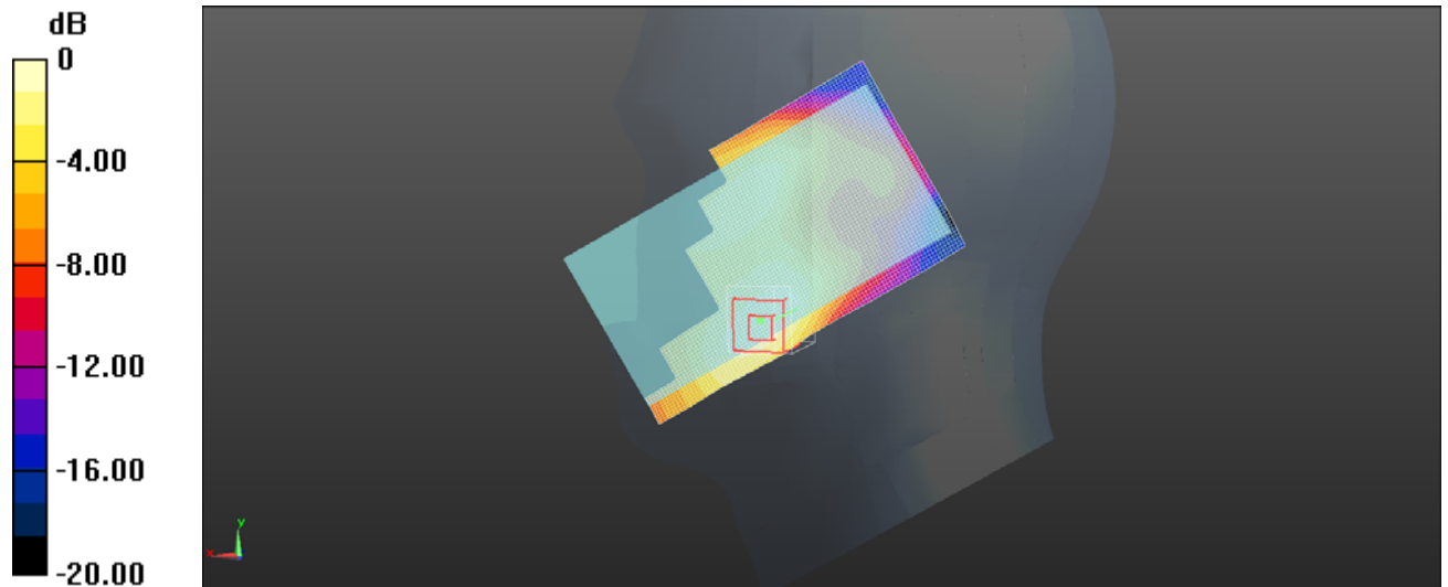
Left Head (PCS1900 Middle Channel)
