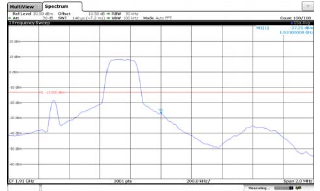
Channel High-1RB#
