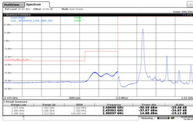
Channel Low-1RB#
