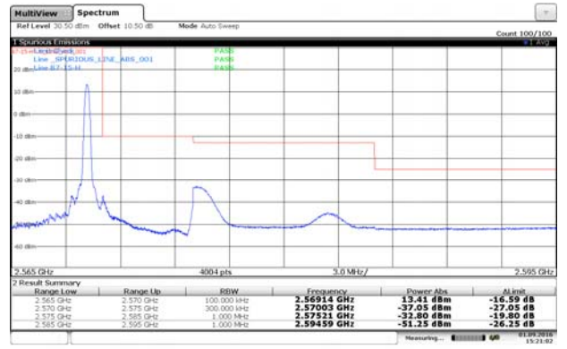
Channel High-1RB#
