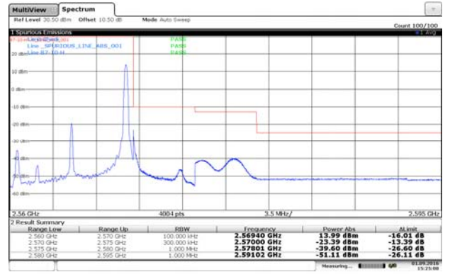
Channel High-1RB#
