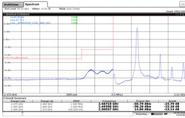
Channel Low-1RB#
