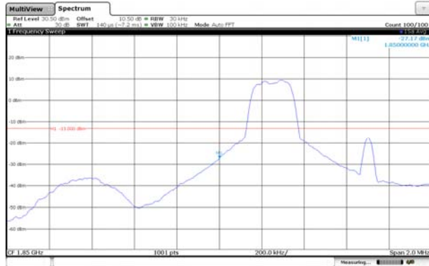
Channel Low-1RB#
