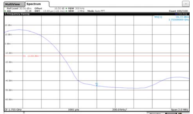
Channel High-1RB#
