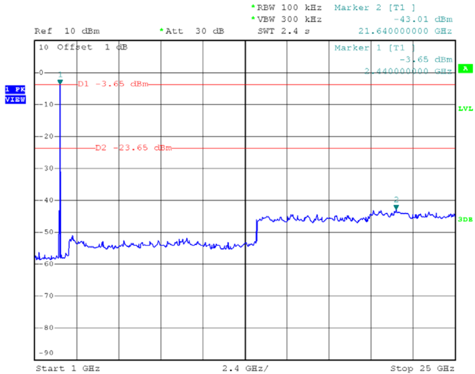
Channel = 19, 1GHz to 25GHz
