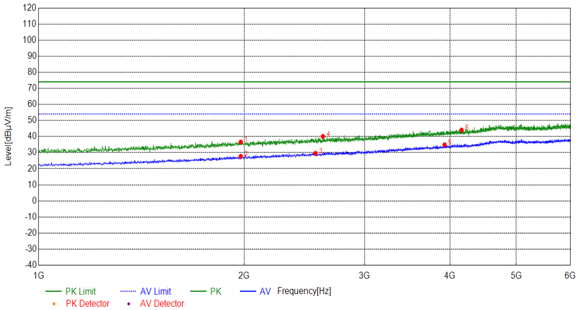
(Plot B: Test Antenna Vertical 1G – 6G)
