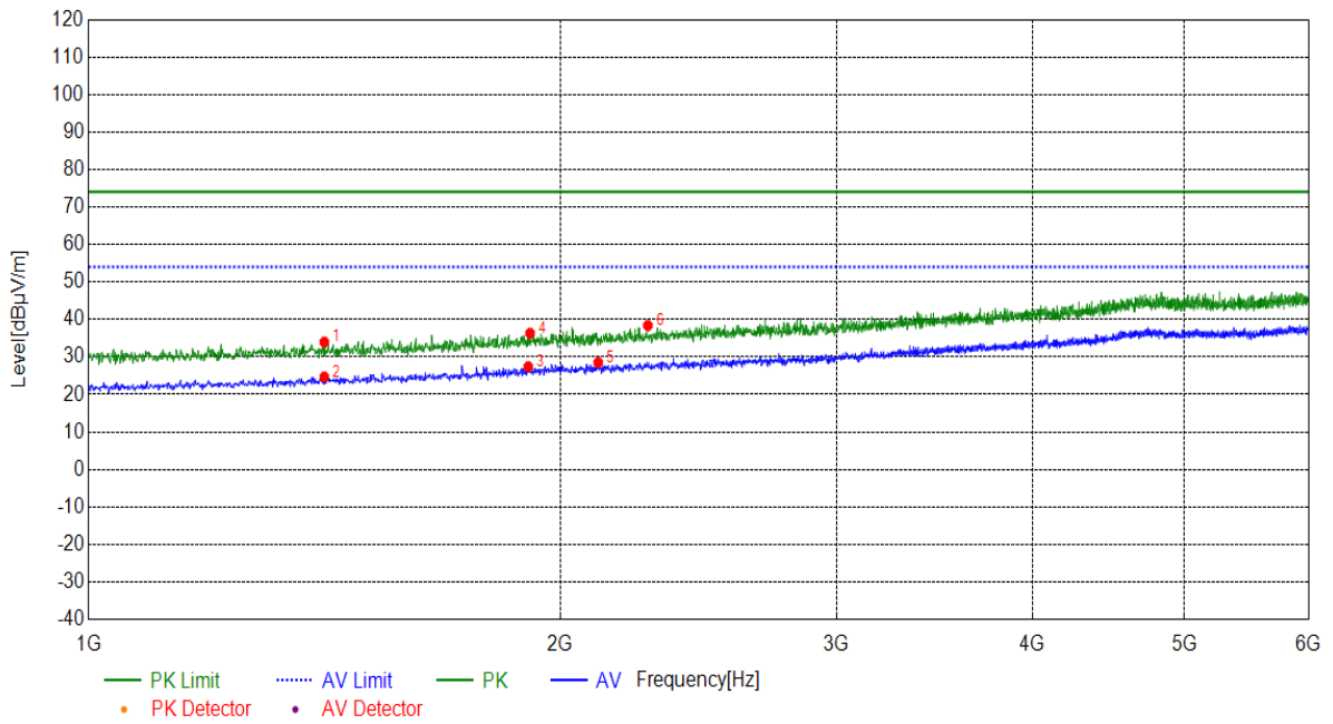
(Plot B: Test Antenna Vertical 1G – 6G)
