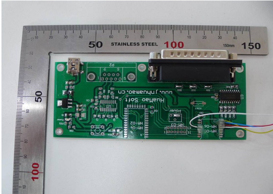
Accessory Circuit HM-DEV-01
