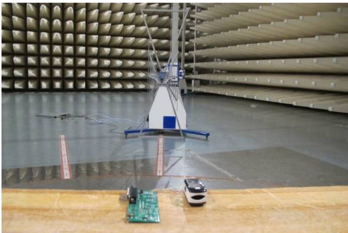
Spurious Radiated Emissions Test setup
