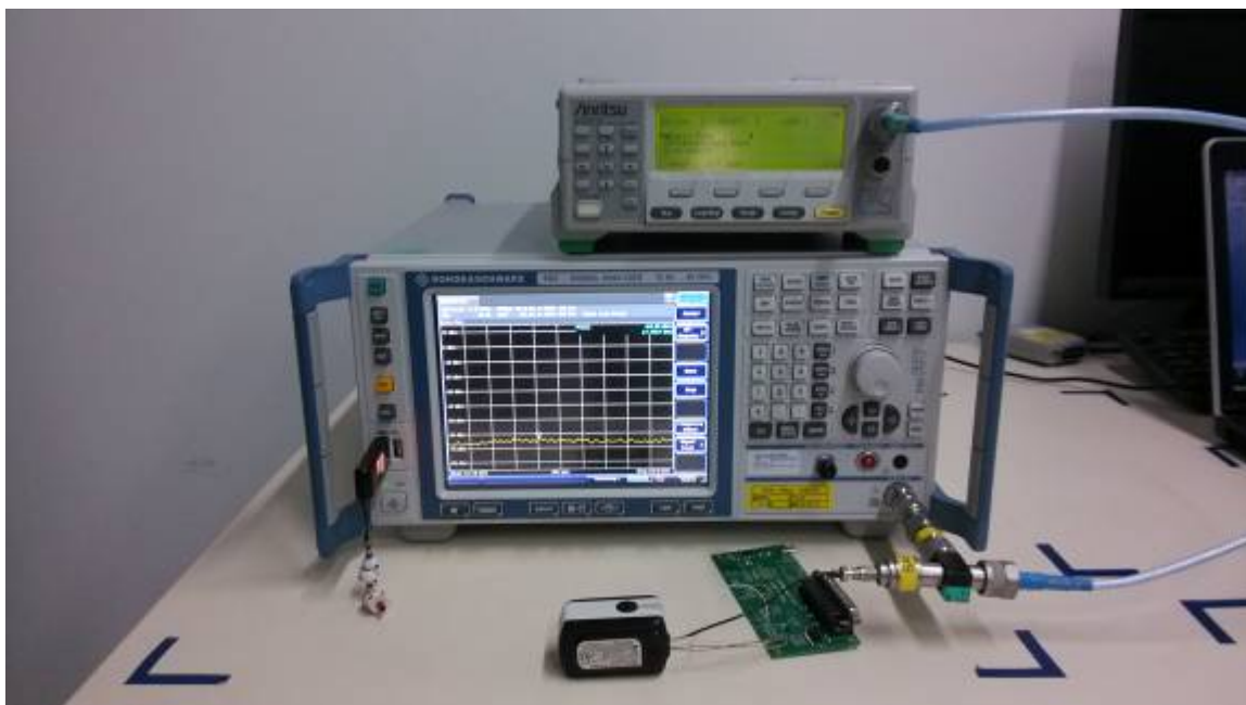
Spurious RF Conducted Emissions Test setup
