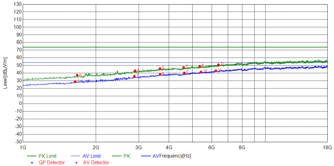
(Plot C: Test Antenna Horizontal 1G – 18G)
