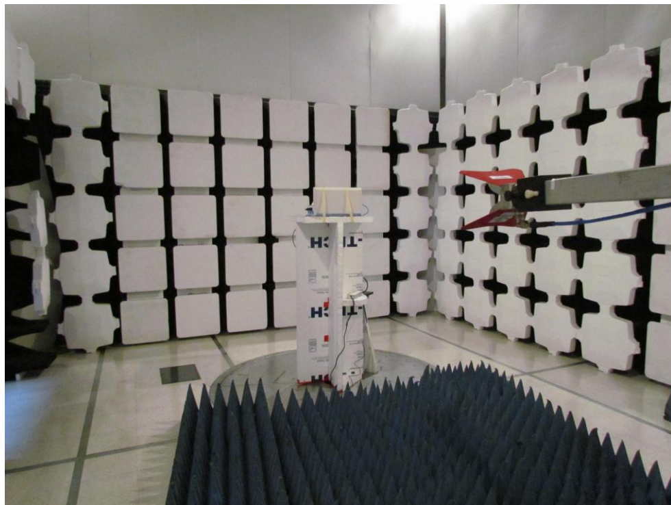
Spurious Emissions: 1-18GHz
