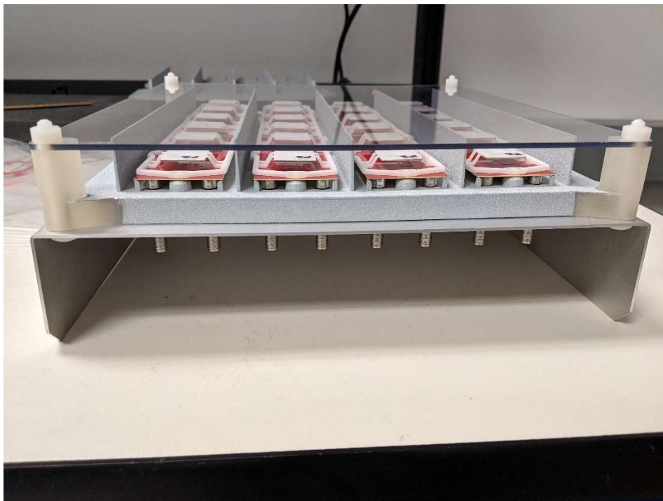
Antenna with Antenna Fixture Photo – Side View
