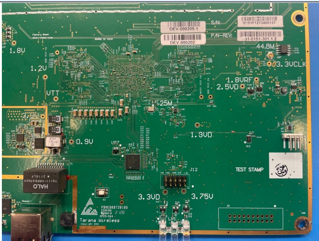
Internal View 6 (Front PCB Detail Veiw_4)
