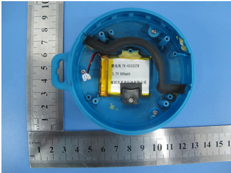
Photo 7 Appearance of Battery
