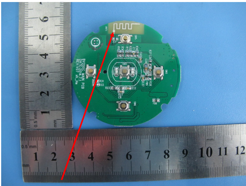
BT(2.4G) Antenna
