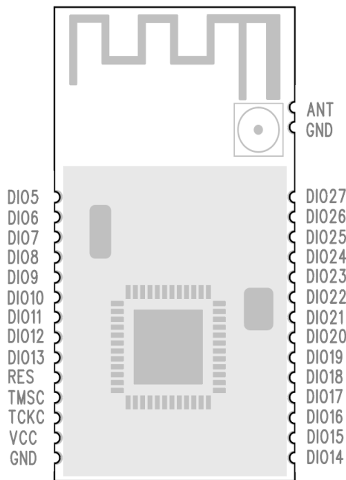
Figure 3. RF-BM-2652P2 pin
