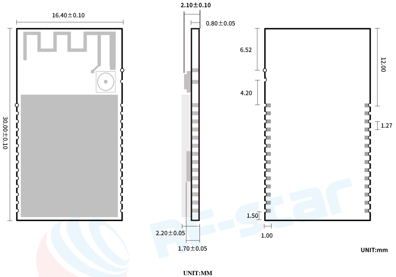
Figure 2. RF-BM-2652P2 size
