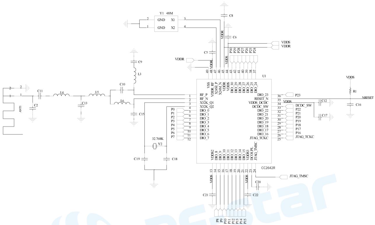
Figure 5. Schematic Diagram of RF-BM-2642B1
