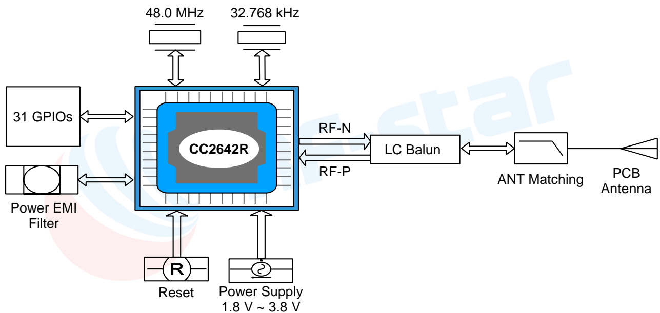
Figure 1. Functional Block Diagram of RF-BM-2642B1
