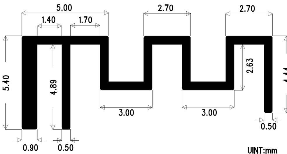
Antenna Dimensions
