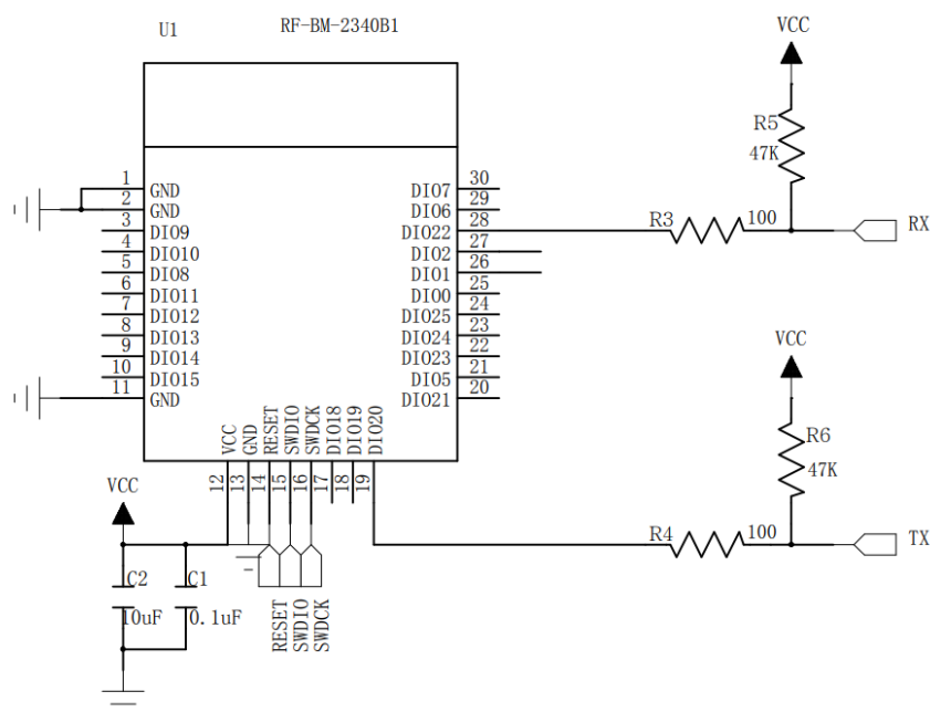
Figure 5. Reference Design of RF-BM-2340B1(I)
