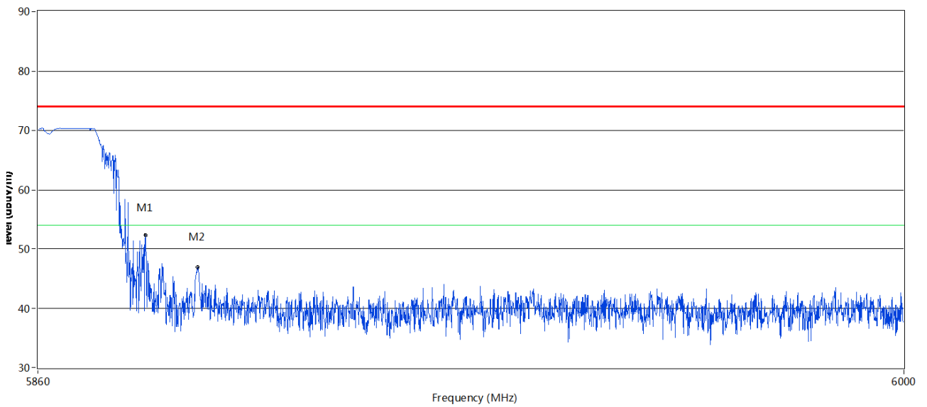
Radiated band-edge_5.8G-Band-edge single-H
