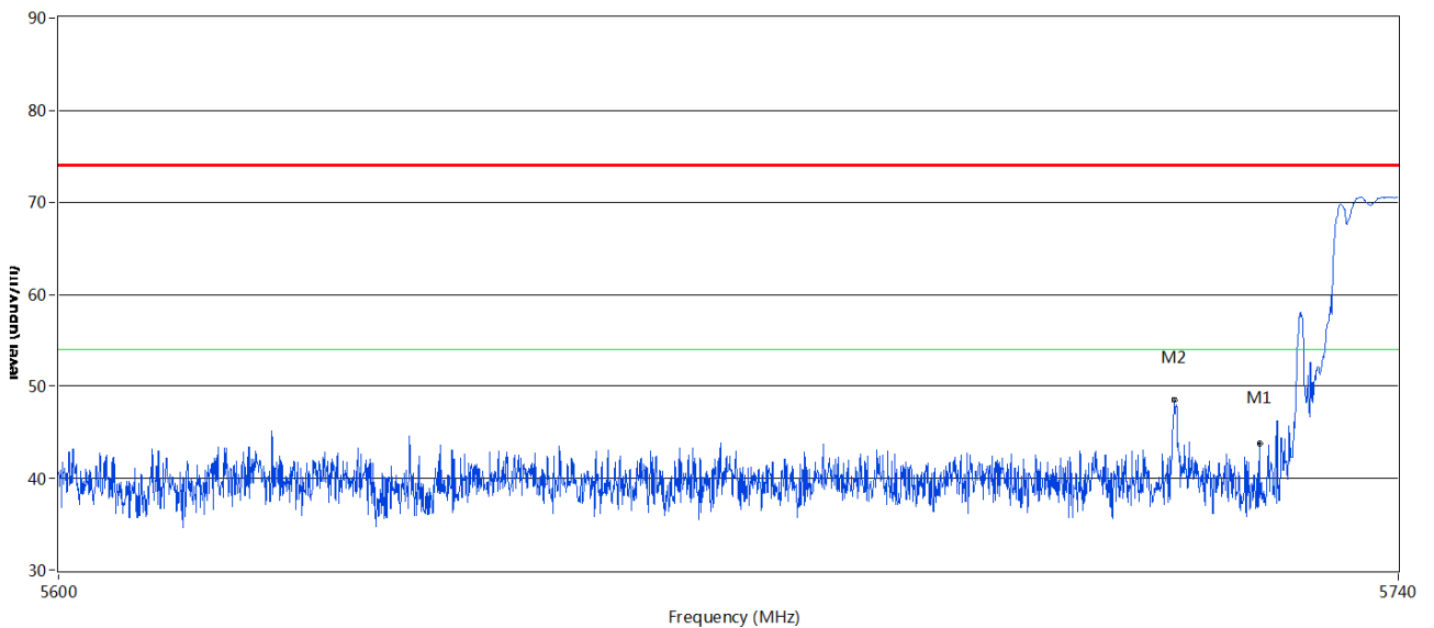
Radiated band-edge_5.8G-Band-edge single-L
