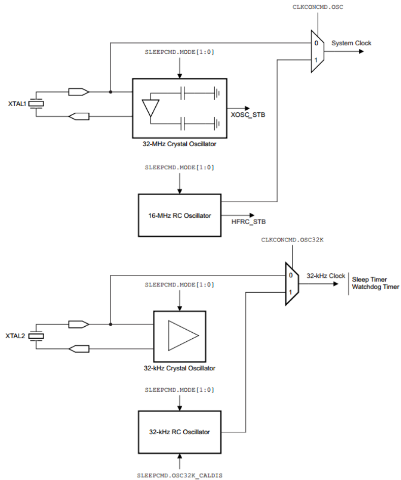
CC2521 Clock System Overview
