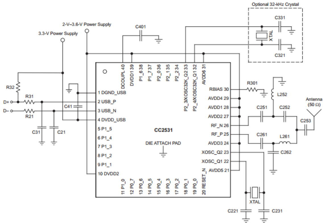
CC2531 Application Circuit
