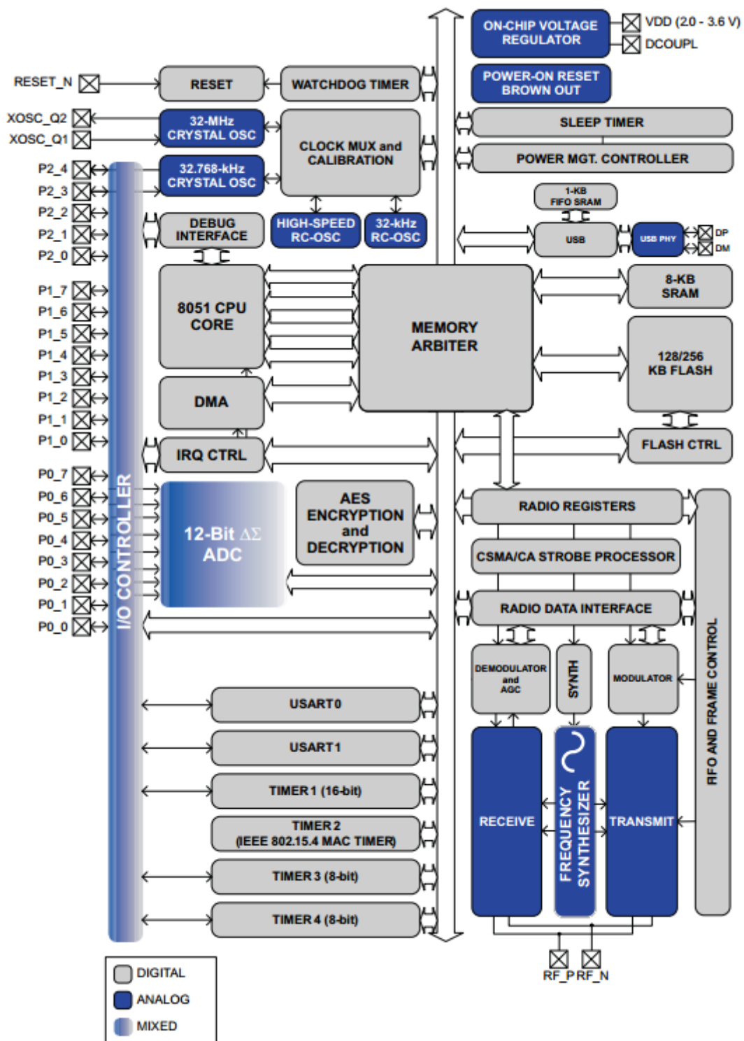
CC2531 Block Diagram
