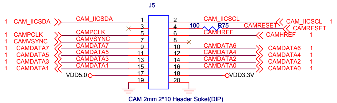
CAM 2mm 2*10 Header Scket(DIP)
