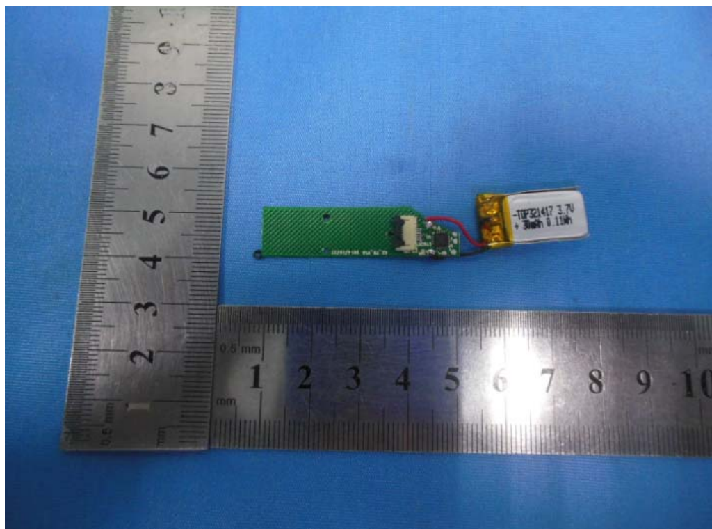
EUT-Battery View
