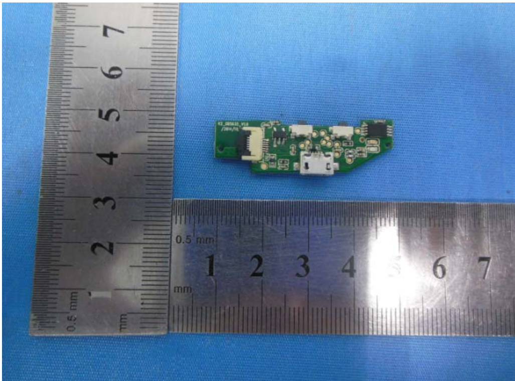
EUT-Battery View
